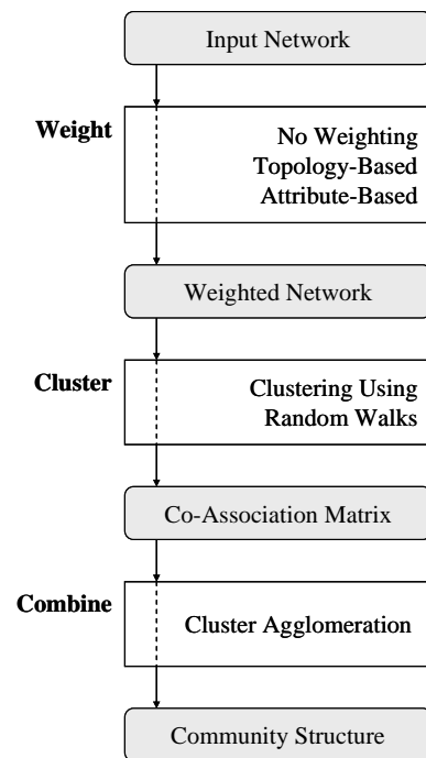
Fig. 1. Algorithm framework for community detection using random walks
