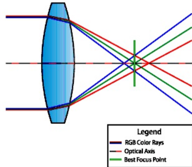
Longitudinal / Axial Chromatic Aberration
