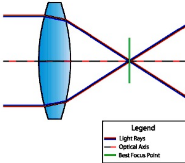
Perfect Lens with no Chromatic Aberration
