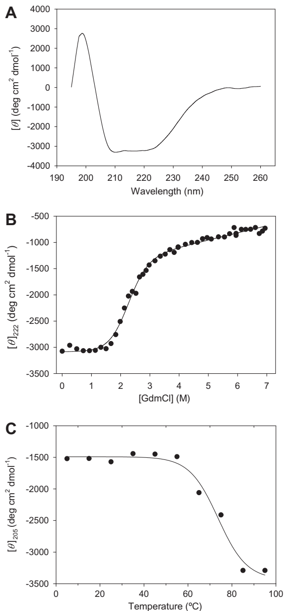
Fig. 4. (A) Far-UV CD spectrum of C-StkP. (B) Monitoring of equilibrium unfolding of C-StkP by CD. (C) Thermal unfolding of C-StkP monitored by following the CD signal at 205 nm. A sigmoidal curve is shown only for presentation purposes and has no thermodynamic meaning.
