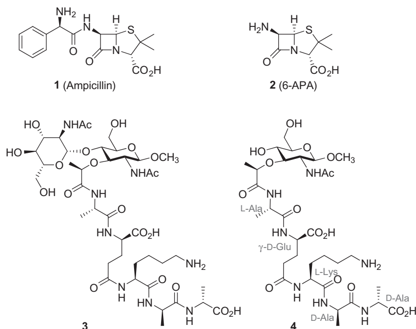
Fig. 1. Chemical structures of ampicillin ( 1 ), 6-aminopenicillanic acid ( 2 ) and synthetic peptidoglycan fragments 3 and 4 .
