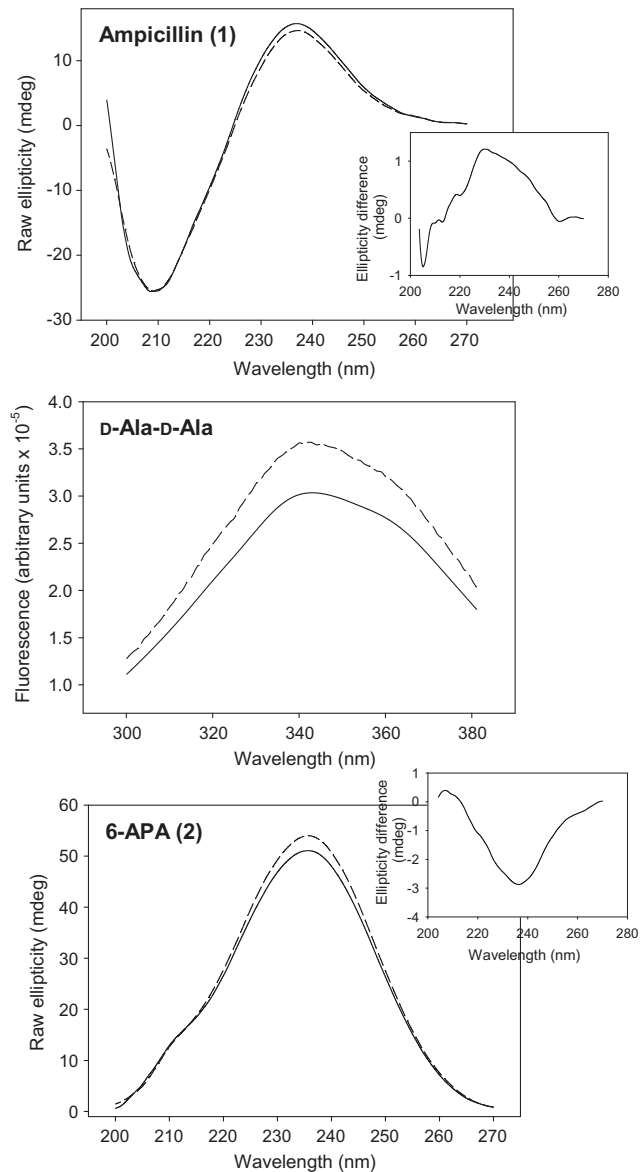
Fig. 5. Upper panel: Interaction of 5.6 \mu M C-StkP with 1 mM ampicillin (1) monitored by CD at 25 ^{\circ} C in 20 mM sodium phosphate, 50 mM NaCl, pH 7.0; the solid line is the experimental spectrum of the complex, and the dashed line is the theoretical spectrum obtained by the sum of the spectra of protein and ligand recorded separately. The inset shows the difference in ellipticity between experimental and theoretical spectra. Experiments were repeated four independent times and a typical result is shown in the figure. Middle panel: Intrinsic fluorescence spectrum of 5.6 \mu M C-StkP (solid line) and 5.6 \mu M C-StkP plus 1 mM D-Ala-D-Ala (dashed line). Lower panel: Interaction of 5.6 \mu M C-StkP with 1 mM 6-APA (2) monitored by CD. Conditions and line patterns as in the upper panel.
