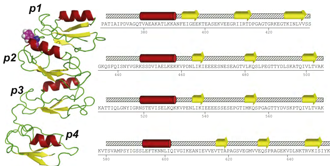
Fig. 3. Left: The three-dimensional homology model of the C-StkP structure, displaying the p1–p4 motifs and the Phe-438 residue (in spacefill representation). Right: Secondary structure assignments to the C-StkP primary structure. \alpha -Helices are represented as red cylinders, \beta -structures are shown as yellow arrows, and other structures (loops and irregular conformations) are displayed as dashed rectangles.
