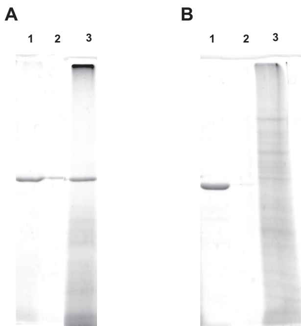
Fig. 6. (A) Interaction of C-StkP with crude peptidoglycan preparations from S. pneumoniae . Lane 1, soluble fraction after binding and centrifugation; lane 2, wash fraction; lane 3, total protein release from incubation of PGN with SDS. (B) Interaction of C-StkP with crude peptidoglycan preparations from S. aureus . Lane 1, soluble fraction after binding and centrifugation; lane 2, wash fraction; lane 3, total protein release from incubation of PGN with SDS.
