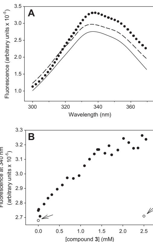
Fig. 7. (A) Interaction of 5.6 \mu M C-StkP[F438W] with 2.5 mM compound 3 or 2.5 mM compound 4 monitored by tryptophan fluorescence spectroscopy. Solid line, protein only; dashed line, protein + 4 ; dotted line, protein + 3 . (B) Fluorescence-monitored titration of C-StkP[F438W] with 3 , followed by fluorescence emission at 340 nm (excitation at 290 nm) (closed circles); effect of compound 3 on the fluorescence of the unrelated protein StyR (open circles marked by arrows). StyR concentration was chosen to be 4.8 \mu M, so that the fluorescence intensity in the absence of ligand matched that of C-StkP[F438W], to facilitate comparison.
