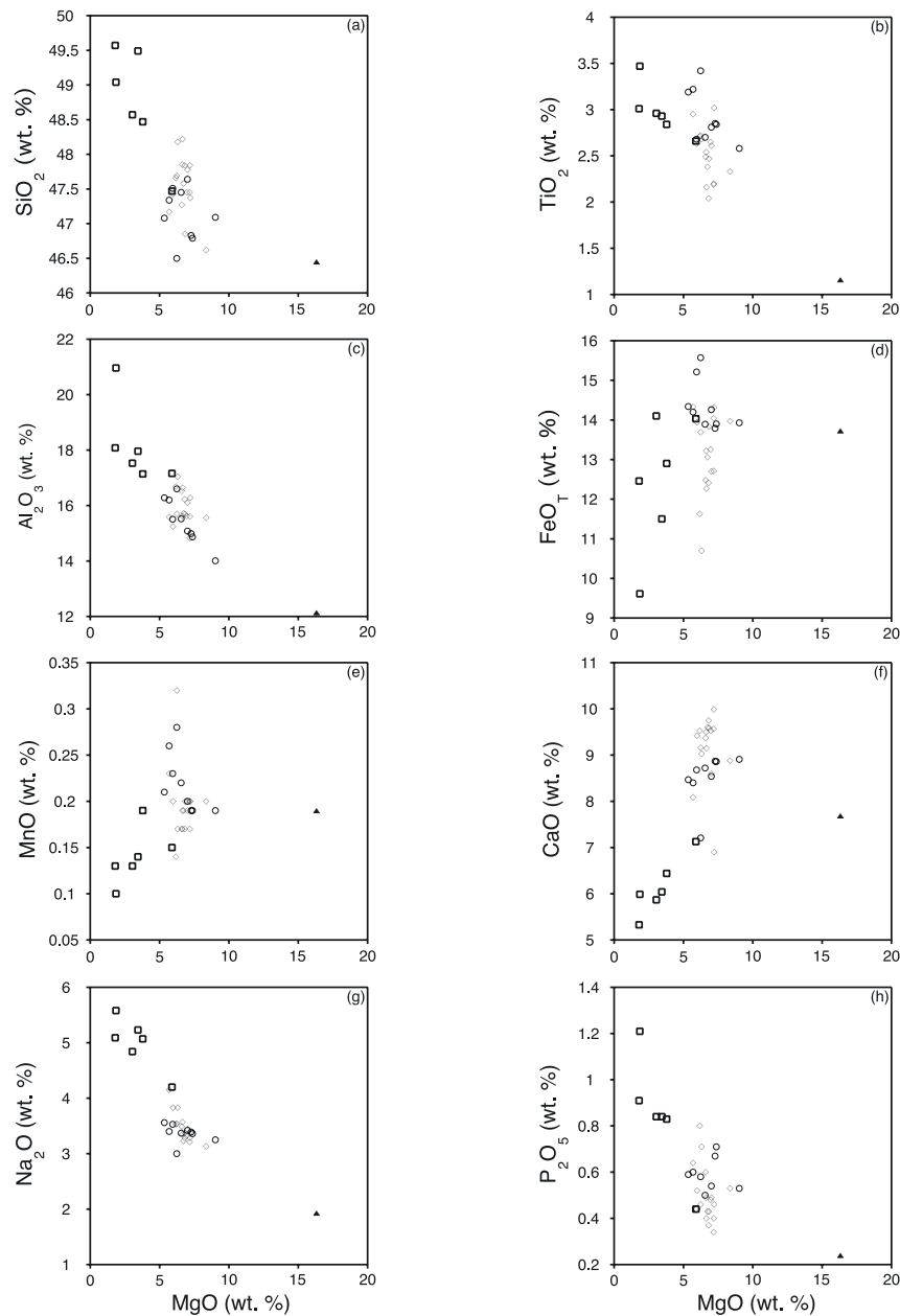
Figure 4. MgO variation diagrams. The clasts from the conglomerate form a roughly linear extension from the Core 6R-2 alkalic basalts ( \text{MgO} = 6.17 and 6.31 wt.%), suggesting that they formed by fractional crystallization of melts of alkalic basalt. Symbols are the same as in Figure 3.
