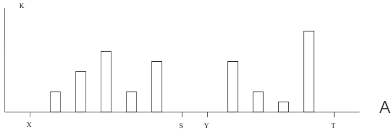
FIGURE 1. The cost of enumerating x into A at stage s is \sum_{x < n < s} 2^{-K_s(n)} and the cost of enumerating x' into A at stage s' is \sum_{x' < n < s'} 2^{-K_{s'}(n)} ; the weights are “disjoint”.
