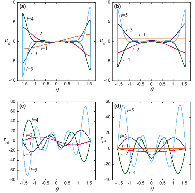
FIG. 2. (Color online) First five sets of functions \psi_{4i}^{\text{odd}} are converted to represent u_\theta and \tau_{r\theta} at r=1 in panels (a, c). Those derived from \psi_{4i}^{\text{even}} are shown in panels (b, d).
