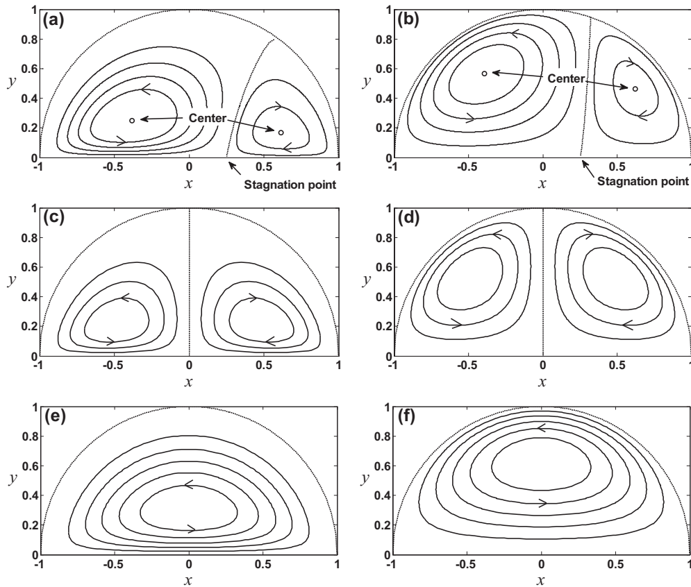
FIG. 4. Respective flow structures generated by the slip velocity, its odd part and its even part depicted in Fig. 3: (a, c, e) under the no-slip condition; (b, d, f) under the free-slip condition. Vortex flow structures in panels (a, b) show converging stagnation points on the bottom surface.
