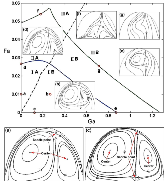
FIG. 6. (Color online) Effects of Fa and Ga on the efficiency of particle trapping at the stagnation point in the free-slip vortex flow of Example 1. Panels (a)–(g) depict different particle dynamics corresponding to the open circles indicated in the upper panel.
