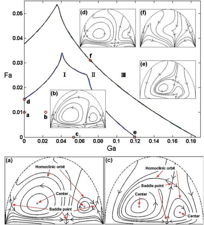
FIG. 5. (Color online) Effects of Fa and Ga on the efficiency of particle trapping at the stagnation point in the no-slip vortex flow of Example 1. Panels (a-f) depict different particle dynamics corresponding to the open circles indicated in the upper panel. Note that the aspect ratio of each semicircle has been varied to exhibit particle dynamics more clearly.
