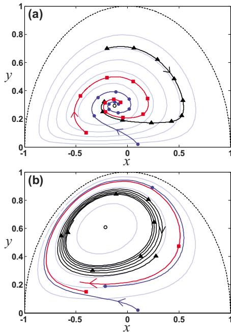
FIG. 8. (Color online) Particle trapping at a point trap (indicated by an open circle) in a single vortex flow (denoted by undertone streamlines) due to a repulsive force from the surface for Example 2: (a) no-slip flow with Z_N=0.675 ; (b) free-slip flow with Z_N=0.675 . Along each particle trajectory, any two adjacent symbols are separated by a time interval of L/U_0 .
