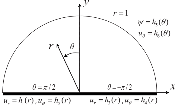
FIG. 1. Geometry of the microfluidic system. In the semicircle, two-dimensional microvortex flow is driven by a nonuniform electrokinetic slip velocity prescribed on the bottom surface.
