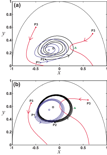
FIG. 11. (Color online) Particle sorting by size via point traps (indicated by open circles and squares) for Example 3: (a) no-slip vortex flow with Ga=0.0105 for P1; (b) free-slip vortex flow with Ga=0.0633 for P1. The point traps for the critical particle motion leading to complete separation are indicated by triangle symbols.
