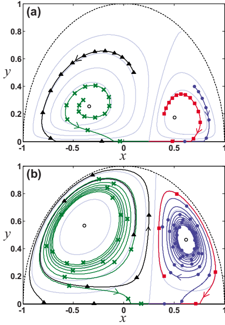
FIG. 7. (Color online) Facilitated particle trapping at the stagnation point due to an attractive NDF force from the bottom surface for Example 1: (a) no-slip vortex flow with Z_N=0.356 ; (b) free-slip vortex flow with Z_N=0.71 . The vortex flow of fluid is denoted by undertone streamlines, the unstable spiral points are indicated by open circles, and particle trajectories are represented by solid lines. In panels (a, b), particles labeled by the same symbol are placed at the same initial locations. Any two adjacent symbols along each particle trajectory are separated by a time interval of L/U_0 .
