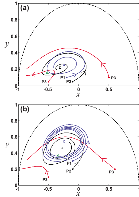
FIG. 10. (Color online) Particle sorting by mobility via point traps (indicated by open circles and squares) for Example 3: (a) no-slip vortex flow with Z_{D1}=0.127 ; (b) free-slip vortex flow with Z_{D1}=0.506 . The point traps for the critical particle motion leading to complete separation are indicated by triangle symbols.
