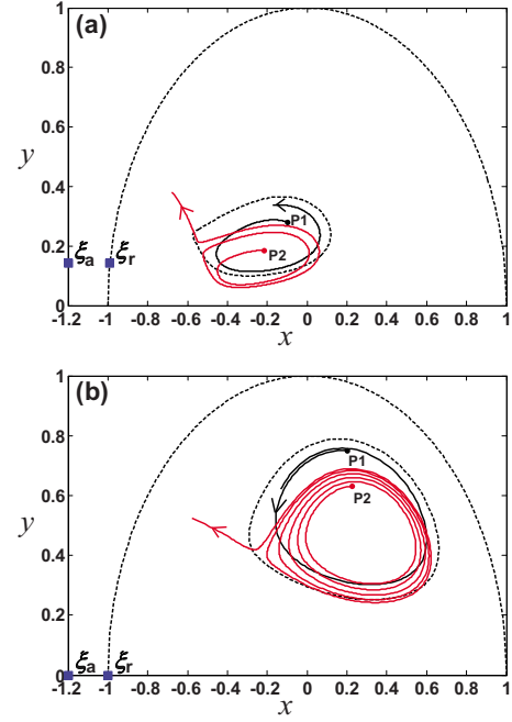
FIG. 12. (Color online) Particle sorting by mobility via limit cycle traps (pictured by the interior dotted lines) for Example 4: (a) no-slip vortex flow with Z_{N1}\xi_r=0.166 ; (b) free-slip vortex flow with Z_{N1}\xi_r=3.97 . For particle P1 in the no-slip vortex flow, a supercritical Hopf bifurcation with \alpha=-3.09 would occur at Z_{N1}\xi_r^*=0.211 and Z_{N1}\xi_a^*=0.529 , whereas for particle P1 in the free-slip vortex flow, a supercritical Hopf bifurcation with \alpha=-0.0842 would occur at Z_{N1}\xi_r^*=4.22 and Z_{N1}\xi_a^*=6.15 .
