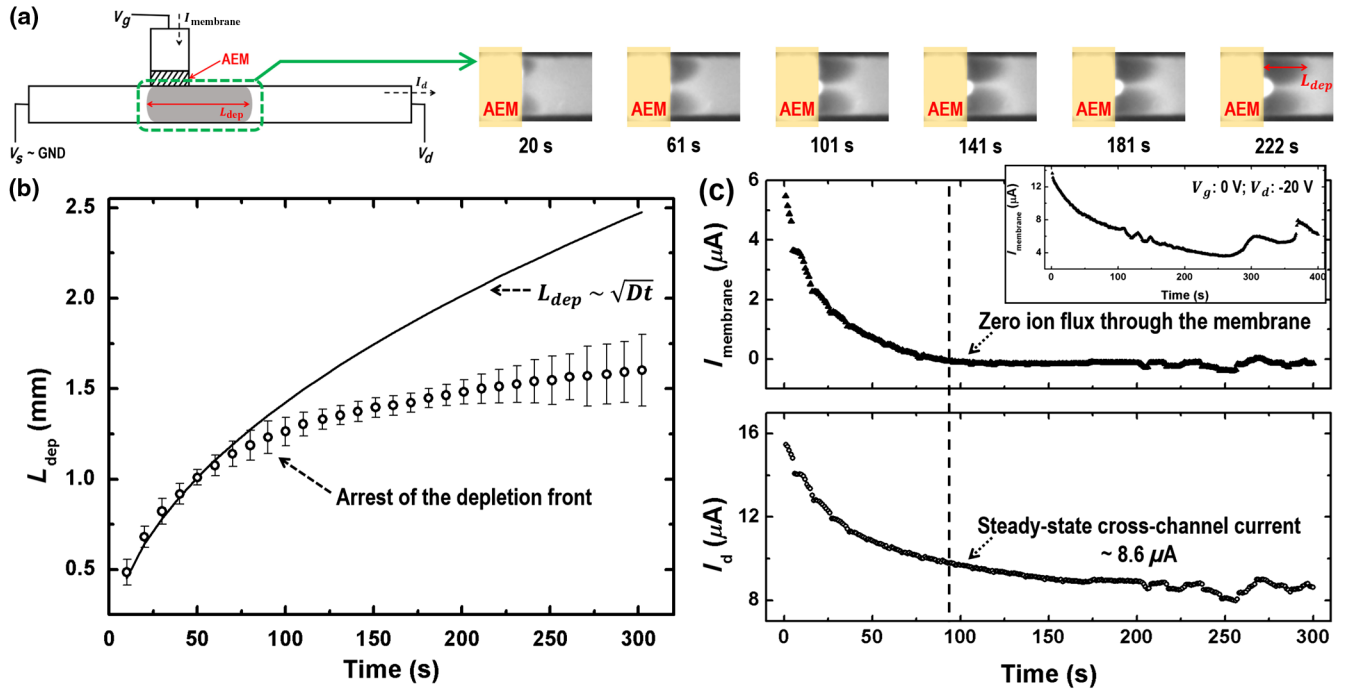
FIG. 2. (a) Fluorescence images of the depletion front at the indicated times. (b) Time evolution of the instantaneous depletion-region length. Also depicted is the (\sqrt{Dt}) scaling as a continuous line. A clear break from the self-similar scaling of the depletion-length growth is observed after 90 s. (c) The charge-generating counterion flux through the AEM ( I_{membrane} ) decreases to zero after 90 s. Correspondingly, the cross-channel current I_d approaches a steady-state value beyond that time. V_d = -15 V and V_g = -2.5 V in the experiment. The inset shows that the transmembrane current I_{membrane} becomes unstable at V_g = 0 V and V_d = -20 V. I_{membrane} cannot vanish to maintain system electroneutrality since the voltage in the cross-channel across the membrane cannot reach the zero gating voltage.
