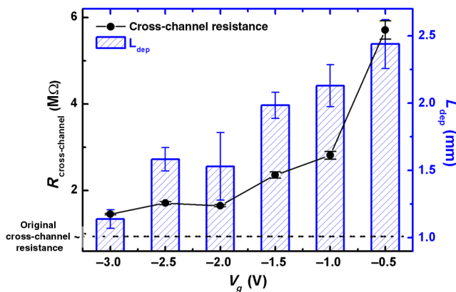
FIG. 3. The ionic resistance of the cross-channel shows strong correlation with the depletion-region length and the gating voltage V_g . V_d = -15\text{V} in all experiments.
