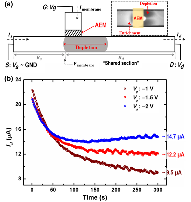
FIG. 1. (a) Schematic of the hybrid ionic path device. (Inset) Fluorescent imaging of simultaneous ion depletion and enrichment on the same side of the AEM membrane. The image is taken from the bottom of the cross-channel, with V_d = -15 V and V_g = -3 V. (b) Temporal evolution of cross-channel current I_d with different V_g 's ( -1 , -1.5 , and -2 V), approaching a different steady-state current for different V_g 's. V_d = -20 V in all three experiments.
