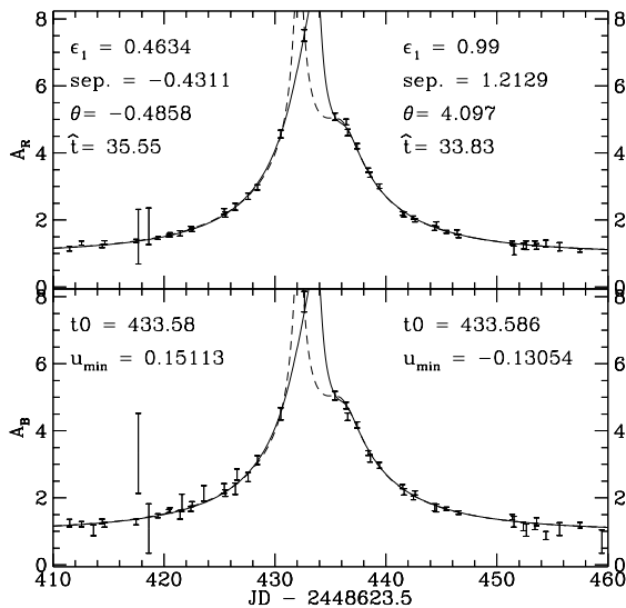
Figure 1. The binary lens fits to the GPE: The solid curve is the small mass fit for \epsilon = 1 - \epsilon_1 = 0.01 , and the lens parameters are shown on the right. The dashed curve is the small separation fit for \epsilon = \epsilon_1 , whose lens parameters are shown on the left. \hat{t} is the transit time of the Einstein ring radius of the total mass, |sep| is the separation, \theta is the angle of the source trajectory with respect to the lens axis where \epsilon_1 is the fractional mass to the positive direction in our convention, and |u_{\min}| is the distance of the source trajectory to the lens axis.
