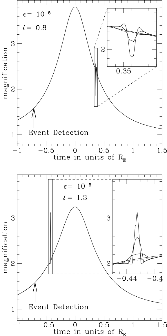
Figure 2. The microlensing signature of earth mass planets orbiting stars of mass 0.3M_{\odot} in the Galactic disk toward the Bulge with separations \ell = 0.8 (upper panel) and \ell = 1.3 (lower panel). The main plots are for a stellar radius of r_s = 0.003 while the insets show the effect of increasing stellar size ( r_s = 0.003, 0.006, 0.013 and 0.03 ).
