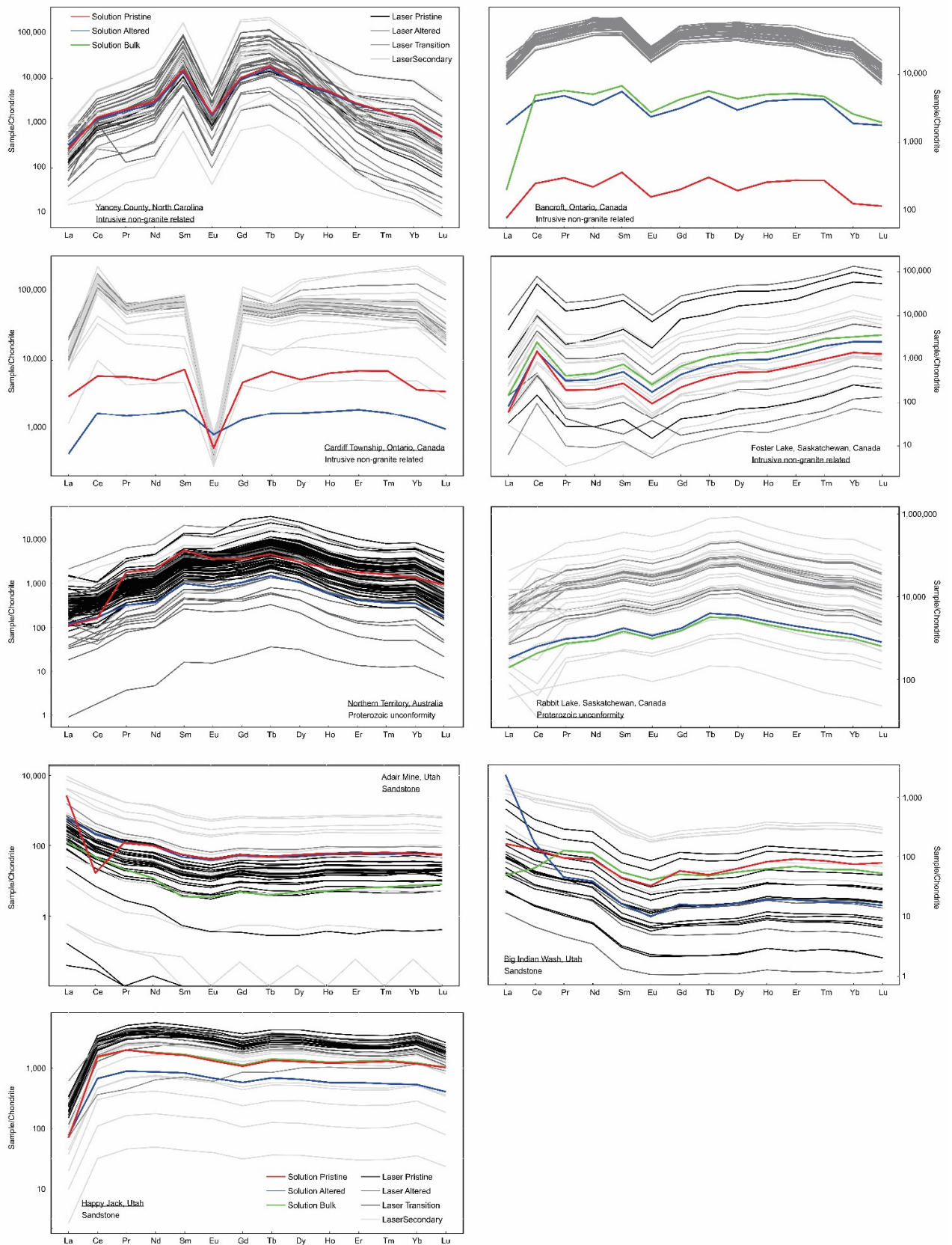
Figure S2. CN-REE Patterns
