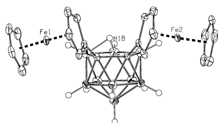
Figure 2. ORTEP plot of Fc^+FcC_2B_9^- ( 3a ) at 50% probability with solvent molecules omitted and only B–H hydrogen atoms shown for clarity. [29]
