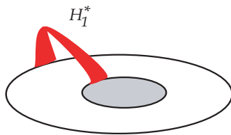
FIGURE 4. Inadmissible 1-handle attachment.
