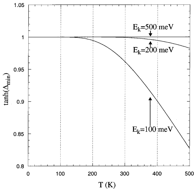
FIG. 10. Effect of temperature for various values of the cell-cell coupling energy E_k . Temperature enters the equation of motion (11) through the function \tanh(\Delta_{\min}) where \Delta_{\min} \approx \hbar E_k / 2k_B T . This function is shown to illustrate how higher values of E_k produce dramatically less temperature sensitivity.
