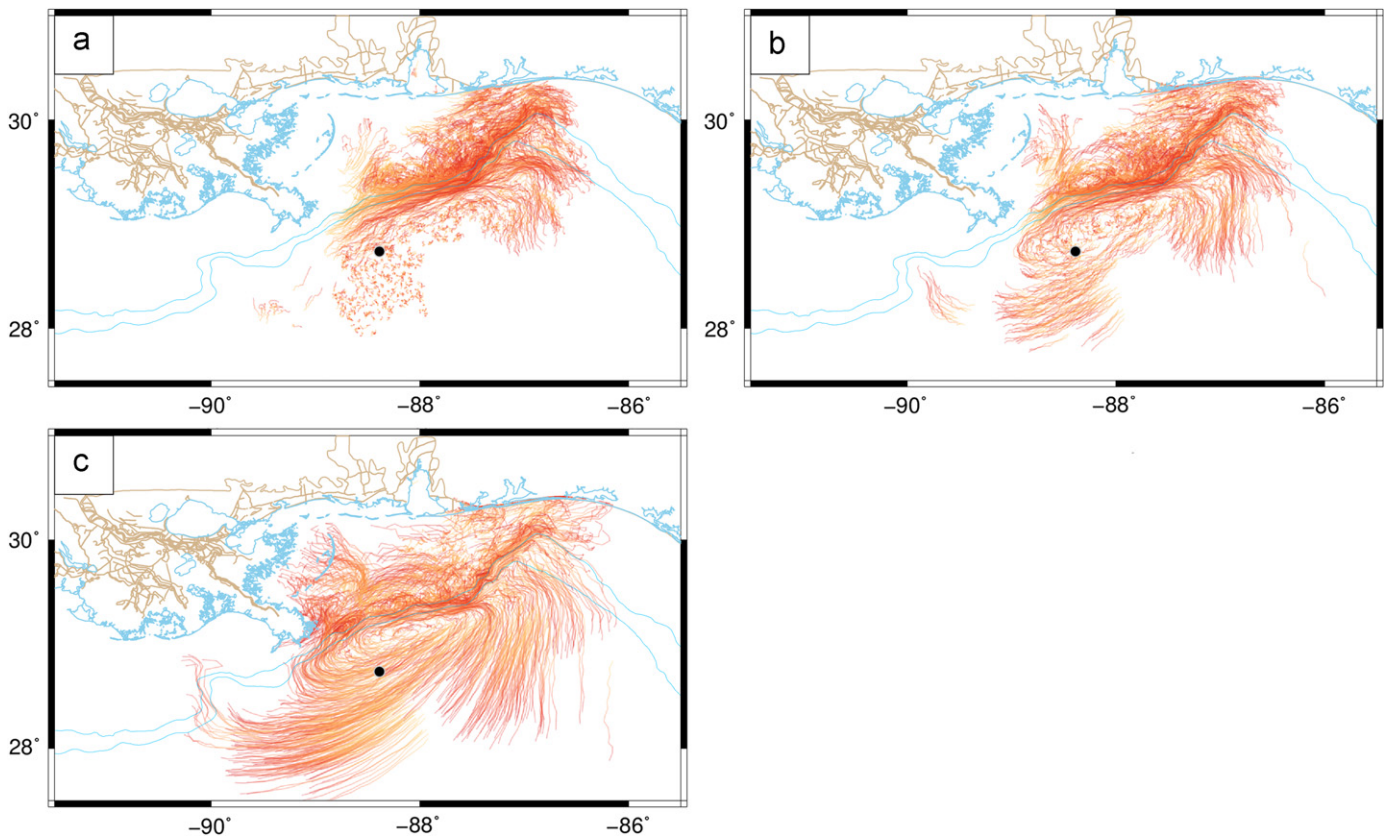
Fig. 14. Sampled predicted particle locations in time during the mid-June period, with forcings from (a) currents only, (b) currents and 1% winds, and (c) currents and 3% winds. Particle movement is shown with the trajectories moving from orange to red. Blue lines indicate the 0 m, 100 m and 200 m bathymetric contours, while brown lines indicate the SL16 internal boundaries. The platform location is also indicated. (For interpretation of the references to color in this figure caption, the reader is referred to the web version of this article.)
