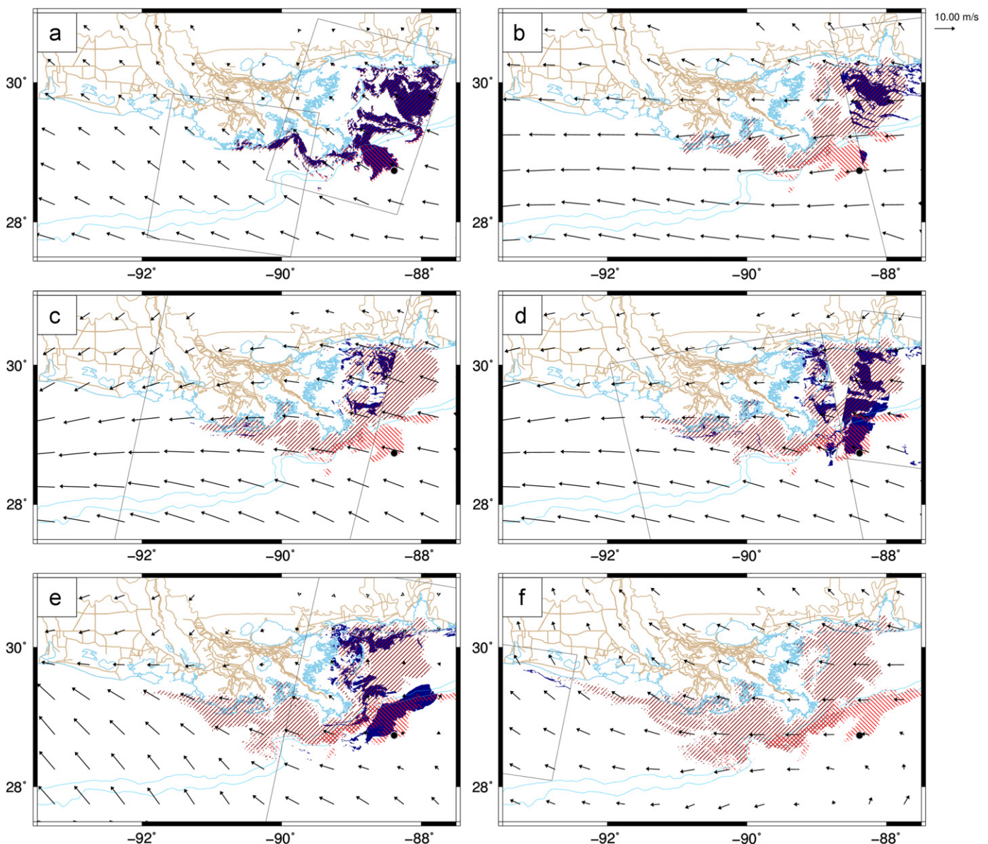
Fig. 21. Comparison of observed (solid blue) and predicted (red hatched) oil extents during the Hurricane Alex time period, with forcing with currents only ( F_c=1 and F_w=0 in Eq. (1)). A distinction is made between oil that started initially in deep water (light red hatching from northwest to southeast) and oil that started initially on the shelf (dark red hatching from northeast to southwest). The panels are (a) the initial conditions on 2010/06/29/0044UTC, (b) conditions after 23 h at 2010/06/29/2332UTC, (c) conditions after 35 h at 2010/06/30/1200UTC, (d) conditions after 47 h at 2010/07/01/0005UTC, (e) conditions after 83 h at 2010/07/02/1156UTC, and (f) conditions after 143 h at 2010/07/05/0008UTC. Vectors are wind velocities ( \text{m s}^{-1} ), and the platform location and the extents of the satellite imagery are also indicated. (For interpretation of the references to color in this figure caption, the reader is referred to the web version of this article.)
