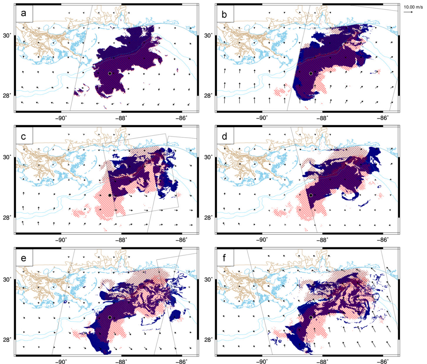
Fig. 11. Comparison of observed (solid blue) and predicted (red hatched) oil extents during the mid-June time period, with forcing with currents only ( F_c=1 and F_w=0 in Eq. (1)). A distinction is made between oil that started initially in deep water (light red hatching from northwest to southeast) and oil that started initially on the shelf (dark red hatching from northeast to southwest). The panels are (a) the initial conditions on 2010/06/13/1548UTC, (b) conditions after 44 h at 2010/06/15/1151UTC, (c) conditions after 92 h at 2010/06/17/1150UTC, (d) conditions after 132 h at 2010/06/19/0341UTC, (e) conditions after 164 h at 2010/06/20/1152UTC, and (f) conditions after 204 h at 2010/06/22/0348UTC. Vectors are wind velocities ( \text{m s}^{-1} ), and the platform location and the extents of the satellite imagery are also indicated. (For interpretation of the references to color in this figure caption, the reader is referred to the web version of this article.)
