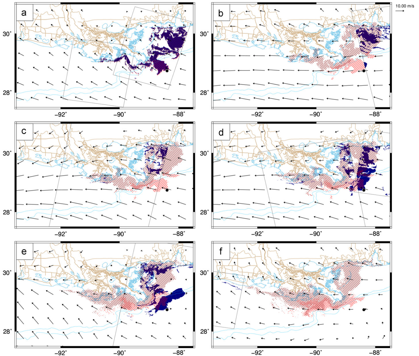
Fig. 22. Comparison of observed (solid blue) and predicted (red hatched) oil extents during the Hurricane Alex time period, with forcing with currents and winds ( F_c=1 and F_w=0.01 in Eq. (1)). A distinction is made between oil that started initially in deep water (light red hatching from northwest to southeast) and oil that started initially on the shelf (dark red hatching from northeast to southwest). The panels are (a) the initial conditions on 2010/06/29/0044UTC, (b) conditions after 23 h at 2010/06/29/2332UTC, (c) conditions after 35 h at 2010/06/30/1200UTC, (d) conditions after 47 h at 2010/07/01/0005UTC, (e) conditions after 83 h at 2010/07/02/1156UTC, and (f) conditions after 143 h at 2010/07/05/0008UTC. Vectors are wind velocities ( \text{m s}^{-1} ), and the platform location and the extents of the satellite imagery are also indicated. (For interpretation of the references to color in this figure caption, the reader is referred to the web version of this article.)
