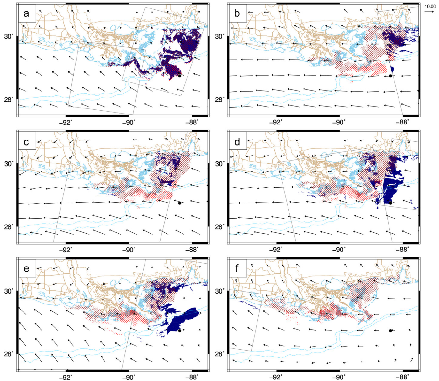
Fig. 23. Comparison of observed (solid blue) and predicted (red hatched) oil extents during the Hurricane Alex time period, with forcing with currents and winds ( F_c=1 and F_w=0.03 in Eq. (1)). A distinction is made between oil that started initially in deep water (light red hatching from northwest to southeast) and oil that started initially on the shelf (dark red hatching from northeast to southwest). The panels are (a) the initial conditions on 2010/06/29/0044UTC, (b) conditions after 23 h at 2010/06/29/2332UTC, (c) conditions after 35 h at 2010/06/30/1200UTC, (d) conditions after 47 h at 2010/07/01/0005UTC, (e) conditions after 83 h at 2010/07/02/1156UTC, and (f) conditions after 143 h at 2010/07/05/0008UTC. Vectors are wind velocities ( \text{m s}^{-1} ), and the platform location and the extents of the satellite imagery are also indicated. (For interpretation of the references to color in this figure caption, the reader is referred to the web version of this article.)
