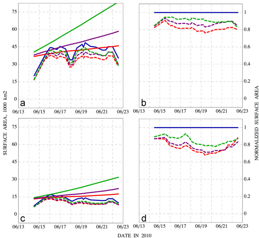
Fig. 17. Total surface areas, using the larger aggregation window, of the observed oil spill (solid blue) and particle tracers (solid red, purple and green) during the mid-June time period, as well as the overlapping areas from the currents/winds scenarios: currents only (dashed red), currents and 1% winds (dashed purple), and currents and 3% winds (dashed green). The panels are (a) areas in 1000 km 2 and (b) normalized areas for oil everywhere, as well as (c) areas in 1000 km 2 and (d) normalized areas for oil only on the continental shelf. In panels (b) and (d), areas are normalized with respect to the observations. (For interpretation of the references to color in this figure caption, the reader is referred to the web version of this article.)
