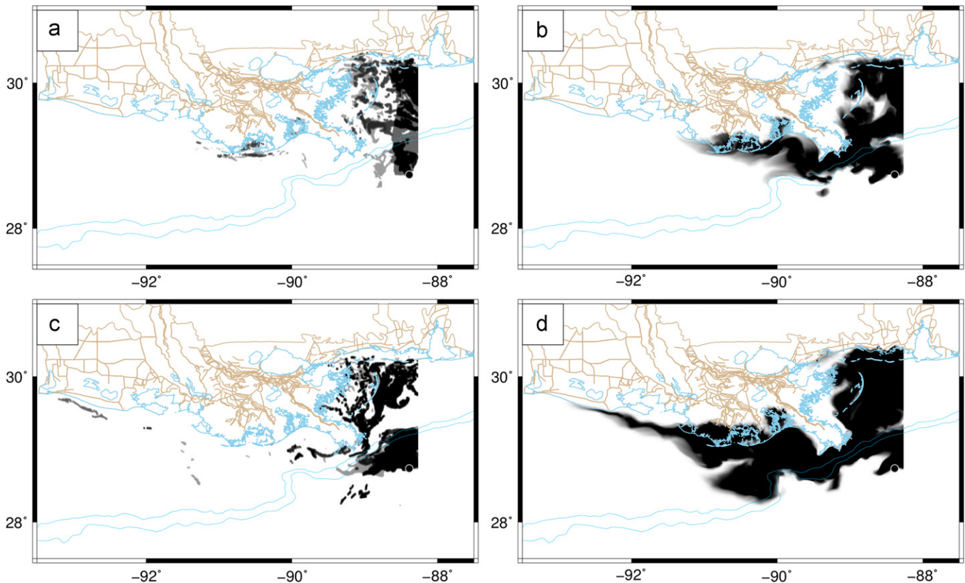
Fig. 26. Samples of aggregation of satellite imagery and predicted particle locations (with currents only) during Alex. Regions without oil are shown in white, while regions with oil are shown in shades of gray and black. Oil east of Mobile Bay is disregarded for this analysis, because it was not present in the initial conditions. The panels are (a) observations and (b) predictions aggregated over a 24 h window around 2010/06/29/2322 UTC, as well as (c) observations and (d) predictions aggregated over a 24 h window around 2010/07/04/1216 UTC. Blue lines indicate the 0 m, 100 m and 200 m bathymetric contours, while brown lines indicate the SL16 internal road/levee boundaries. The platform location is also indicated. (For interpretation of the references to color in this figure caption, the reader is referred to the web version of this article.)
