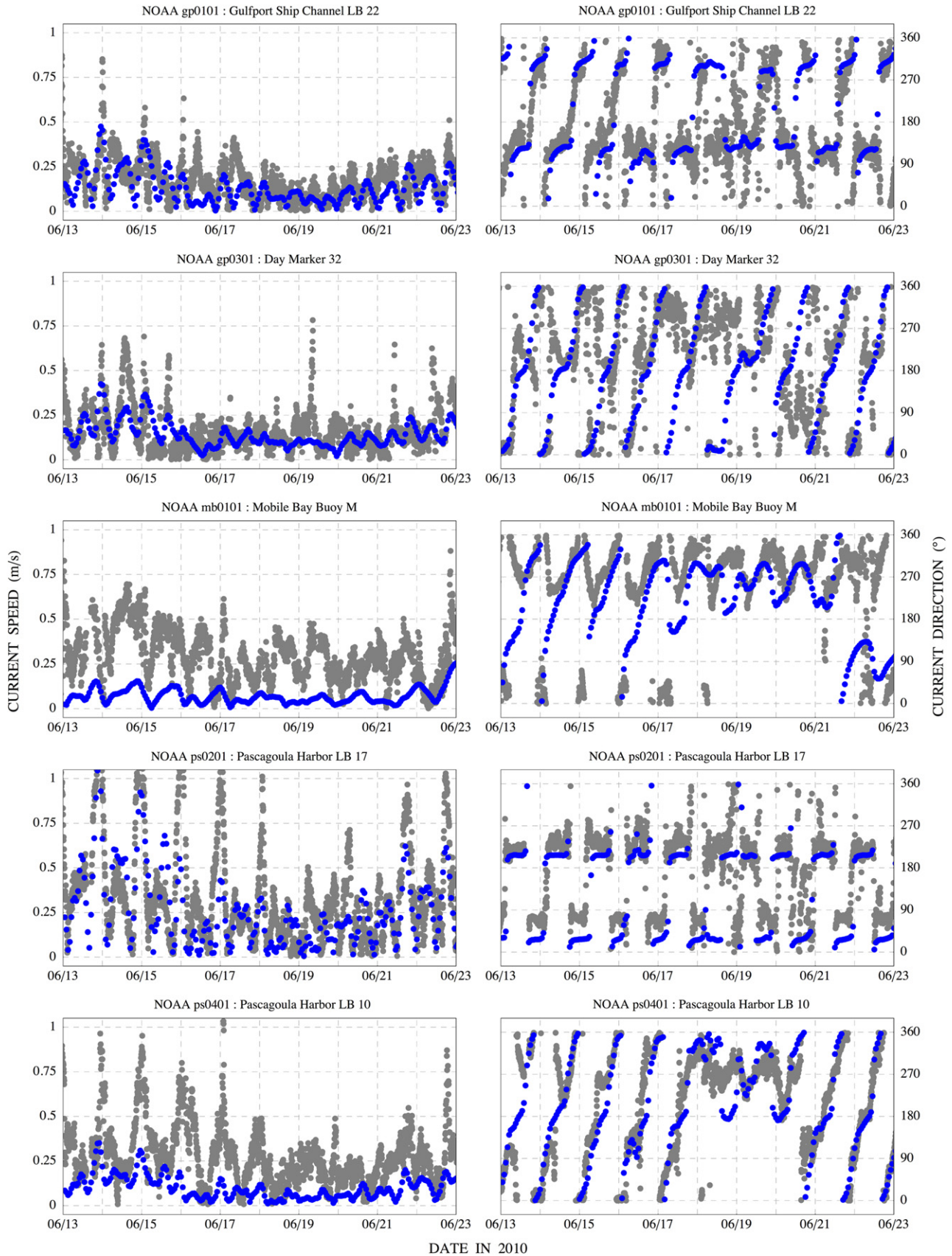
Fig. 10. Current speeds ( \text{m s}^{-1} ) and directions ( ^{\circ} , measured clockwise from true north) at selected NOAA stations during the mid-June time period. Gray circles are measured data from NOAA, while blue circles are predicted ADCIRC currents. Station locations are shown spatially in Fig. 7. (For interpretation of the references to color in this figure caption, the reader is referred to the web version of this article.)
