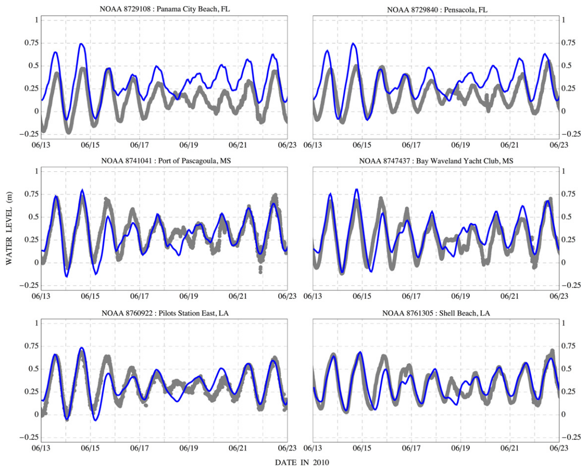
Fig. 9. Water levels (m, relative to NAVD88 (2004.65)), at selected NOAA stations during the mid-June time period. Gray circles are measured data from NOAA, while solid blue lines are predicted ADCIRC water levels. Station locations are shown spatially in Fig. 7. (For interpretation of the references to color in this figure caption, the reader is referred to the web version of this article.)
