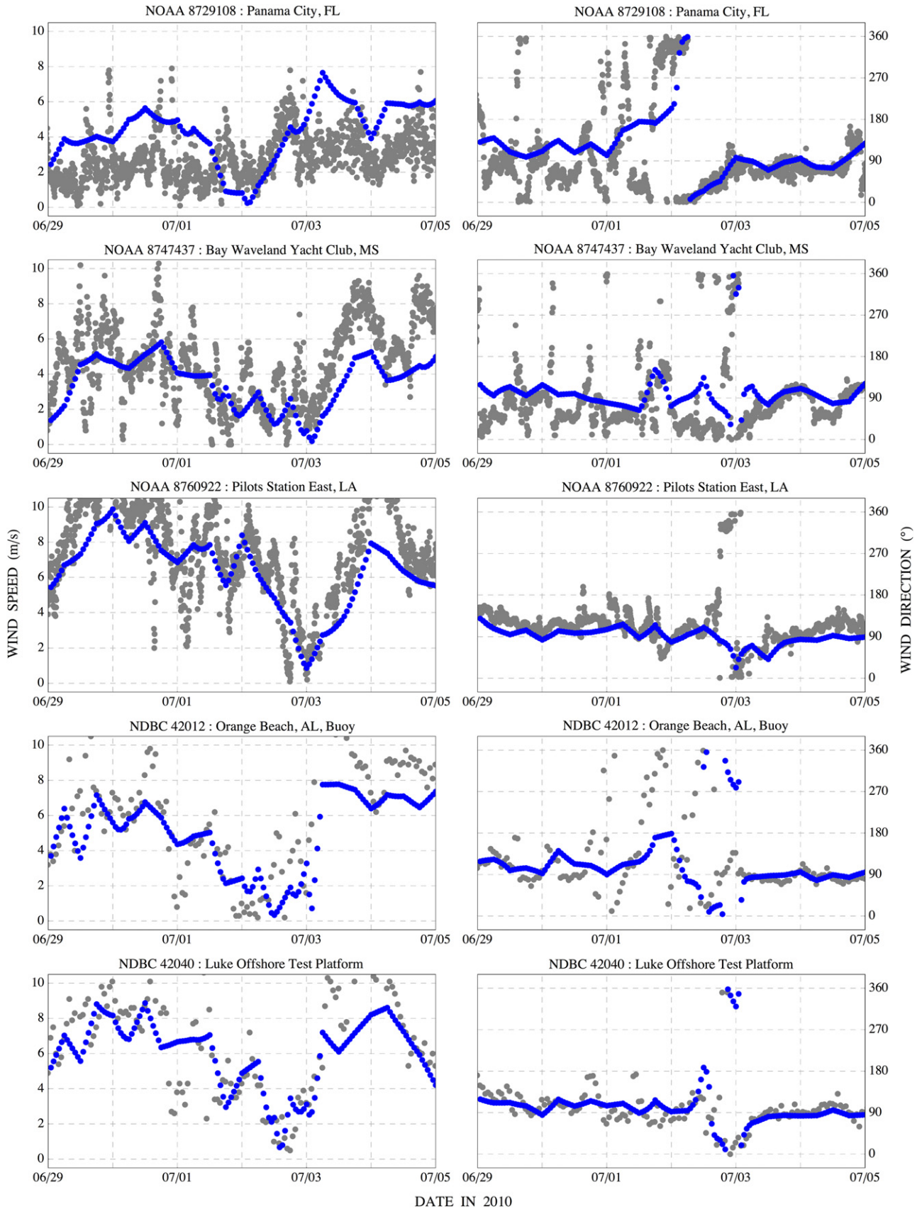
Fig. 18. Wind speeds ( \text{m s}^{-1} ) and directions ( ^\circ , measured clockwise from true north) at selected NOAA stations and NDBC platforms during the Alex time period. Gray circles are measured data from NOAA and NDBC, while blue circles are wind input to SWAN+ADCIRC. Station locations are shown spatially in Fig. 7. (For interpretation of the references to color in this figure caption, the reader is referred to the web version of this article.)
