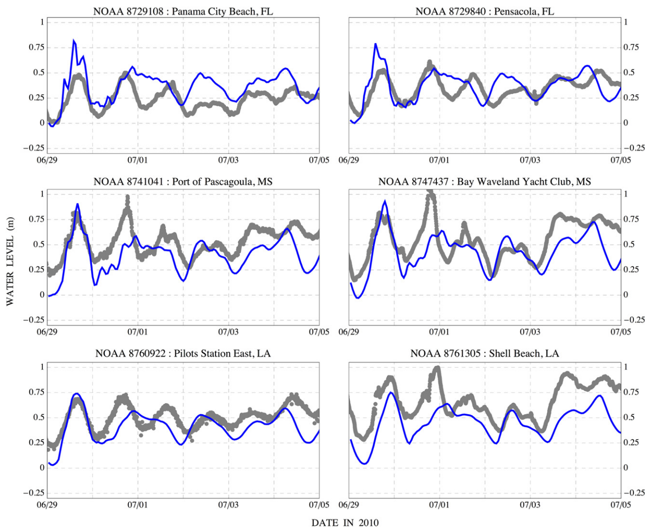
Fig. 19. Water levels (m, relative to NAVD88 (2004.65)), at selected NOAA stations during the Alex time period. Gray circles are measured data from NOAA, while solid blue lines are predicted ADCIRC water levels. Station locations are shown spatially in Fig. 7. (For interpretation of the references to color in this figure caption, the reader is referred to the web version of this article.)
