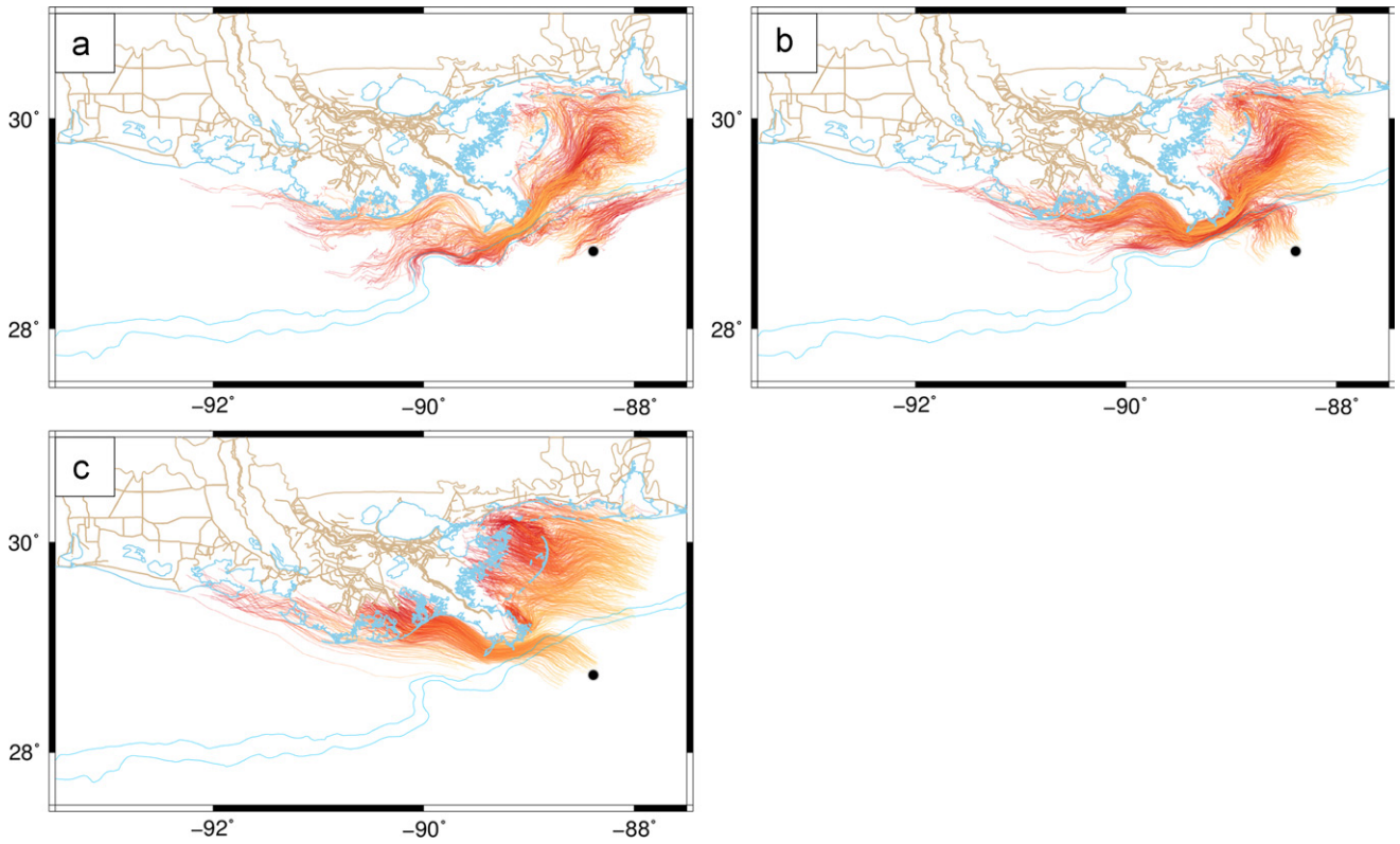
Fig. 24. Sampled predicted particle locations in time during Alex, with forcings from (a) currents only, (b) currents and 1% winds, and (c) currents and 3% winds. Particle movement is shown with the trajectories moving from orange to red. Blue lines indicate the 0 m, 100 m and 200 m bathymetric contours, while brown lines indicate the SL16 internal road/levee boundaries. (For interpretation of the references to color in this figure caption, the reader is referred to the web version of this article.)
