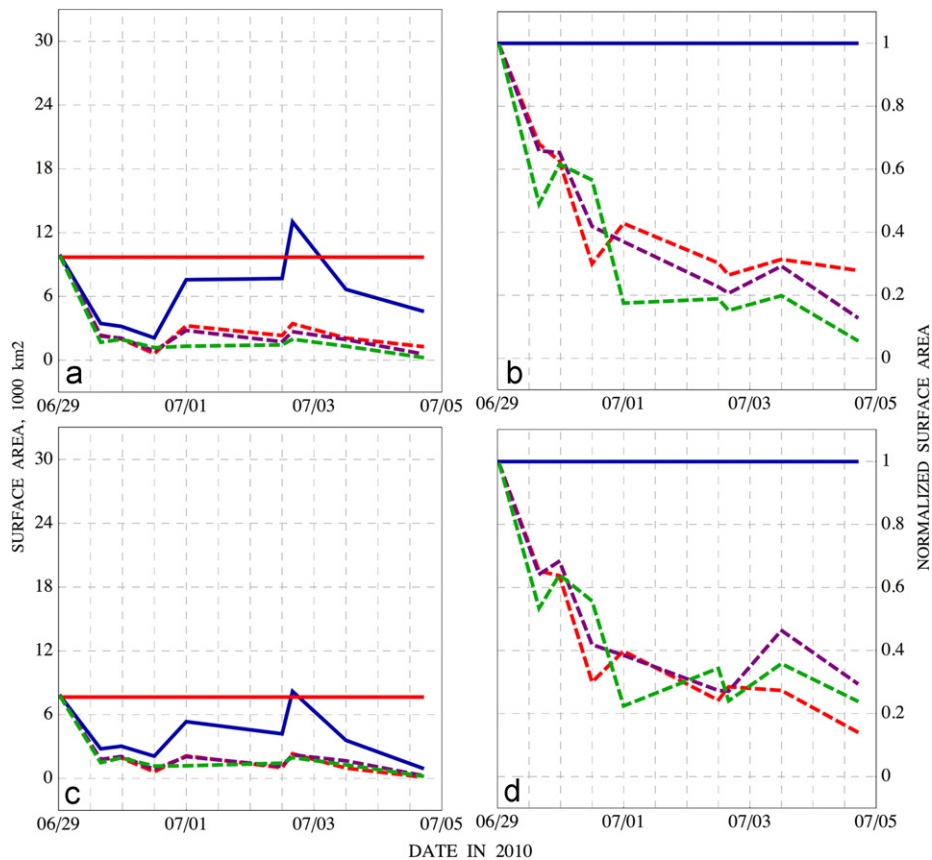
Fig. 25. Total surface areas of the observed oil spill (solid blue) and particle tracers (solid red) during Alex, as well as the overlapping areas from the currents/winds scenarios: currents only (dashed red), currents and 1% winds (dashed purple), and currents and 3% winds (dashed green). The panels are (a) areas in 1000 km 2 and (b) normalized areas for oil everywhere, as well as (c) areas in 1000 km 2 and (d) normalized areas for oil only on the continental shelf. In panels (b) and (d), areas are normalized with respect to the observations. (For interpretation of the references to color in this figure caption, the reader is referred to the web version of this article.)
