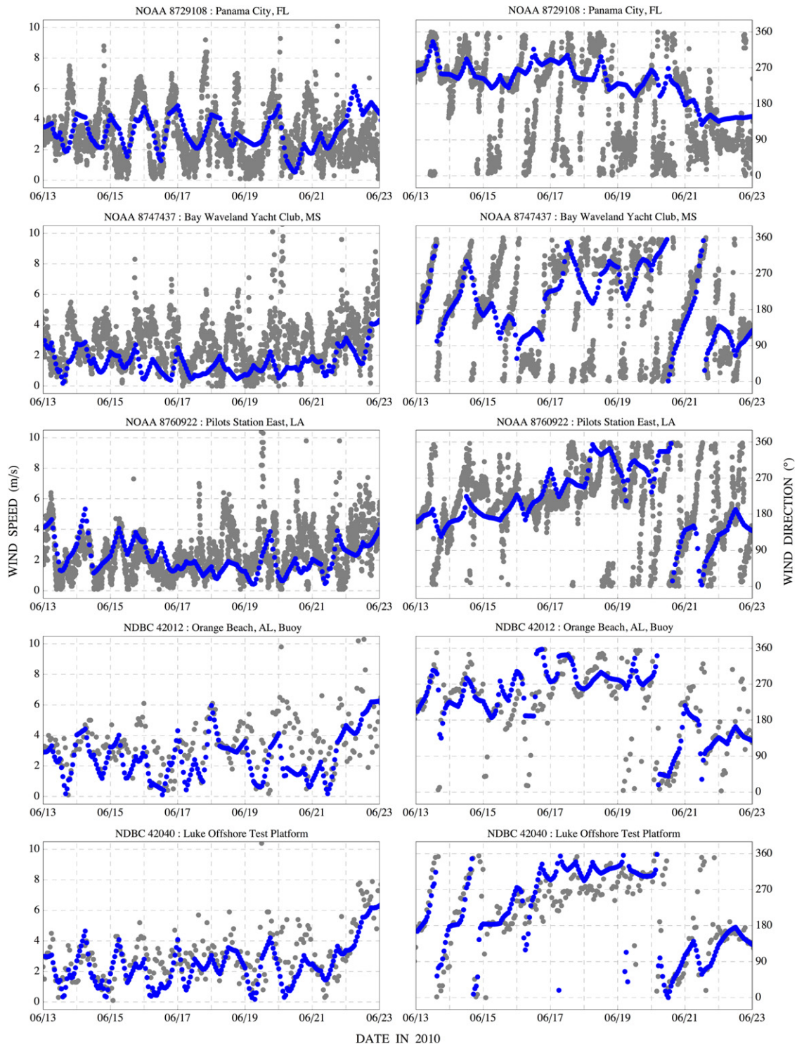
Fig. 8. Wind speeds ( \text{m s}^{-1} ) and directions ( ^{\circ} , measured clockwise from true north) at selected NOAA stations and NDBC platforms during the mid-June time period. Gray circles are measured data from NOAA and NDBC, while blue circles are wind input to SWAN+ADCIRC. Station locations are shown spatially in Fig. 7. (For interpretation of the references to color in this figure caption, the reader is referred to the web version of this article.)
