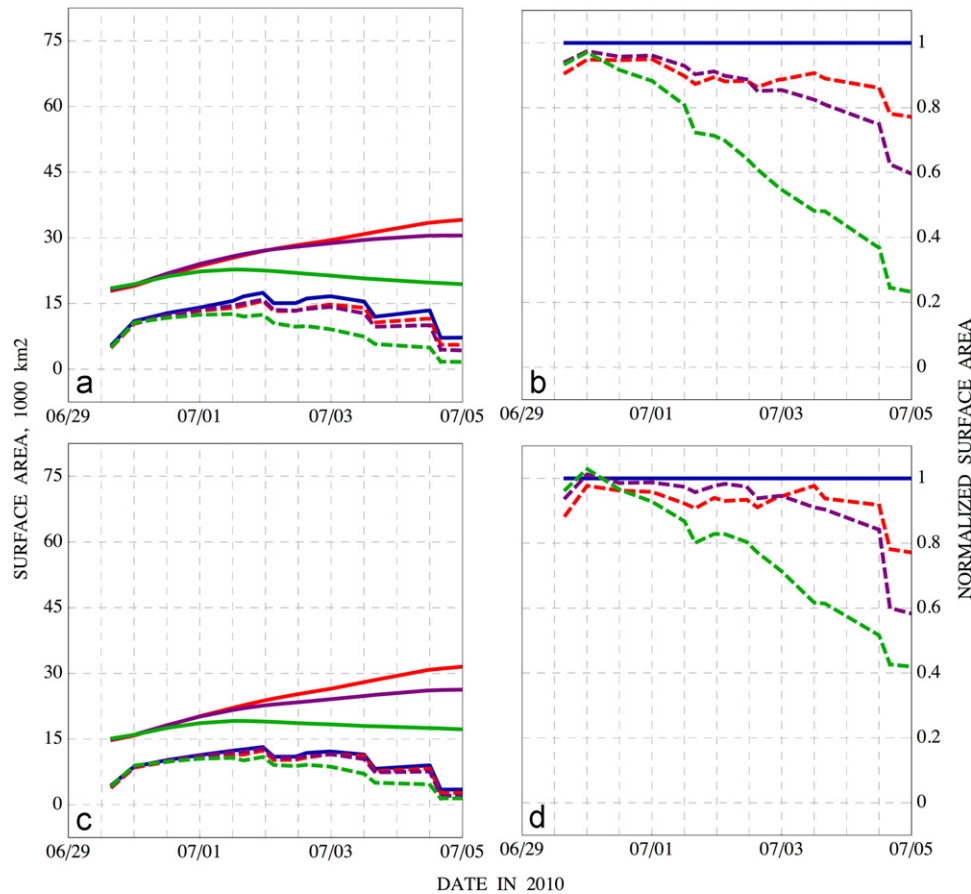
Fig. 27. Total surface areas, using the larger aggregation window, of the observed oil spill (solid blue) and particle tracers (solid red, purple and green) during Alex, as well as the overlapping areas from the currents/winds scenarios: currents only (dashed red), currents and 1% winds (dashed purple), and currents and 3% winds (dashed green). The panels are (a) areas in 1000 km 2 and (b) normalized areas for oil everywhere, as well as (c) areas in 1000 km 2 and (d) normalized areas for oil only on the continental shelf. In panels (b) and (d), areas are normalized with respect to the observations. (For interpretation of the references to color in this figure caption, the reader is referred to the web version of this article.)
