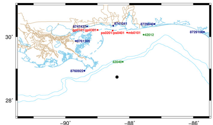
Fig. 7. Locations of the NOAA stations that measured winds and water levels (blue) and currents (red), and the NDBC platforms (green) used in the validation of winds and circulation. Blue lines indicate the 0 m, 100 m and 200 m bathymetric contours, while brown lines indicate the SL16 internal road/levee boundaries. The platform location is also indicated. (For interpretation of the references to color in this figure caption, the reader is referred to the web version of this article.)
