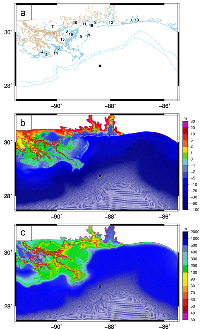
Fig. 3. SL16 mesh in the northern Gulf of Mexico, with panels of (a) geographic locations indicated by numbers identified in Table 1, (b) bathymetry/topography (m, relative to NAVD88 2004.65), and (c) mesh resolution (m). The platform location is also indicated.
