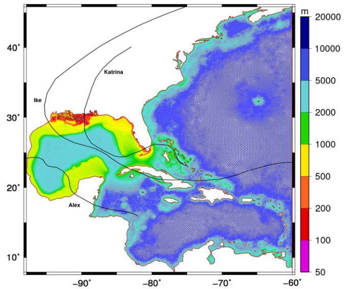
Fig. 2. Mesh resolution (m) of the SL16 mesh. Hurricane tracks are shown in black lines.
