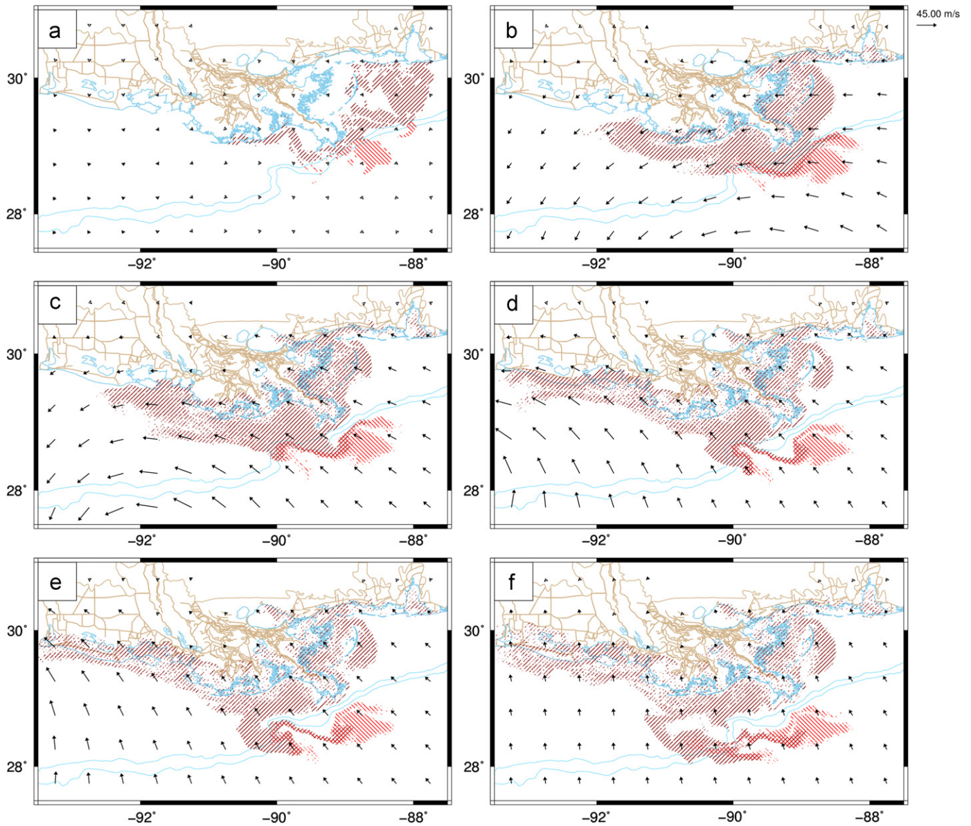
Fig. 29. Hypothetical (red hatched) oil extents during Hurricane Ike (2008), with initial conditions to match the observed oil extents on 2010/06/29/0044UTC, and with forcing with currents only ( F_c=1 and F_w=0 in Eq. (1)). A distinction is made between oil that started initially in deep water (light red hatching from northwest to southeast), and oil that started initially on the shelf (dark red hatching from northeast to southwest). The panels are (a) the initial conditions applied to 2008/09/05/1300UTC, (b) conditions after 155 h at 2008/09/12/0000UTC, (c) conditions after 167 h at landfall on 2008/09/12/1200UTC, (d) conditions after 179 h at 2008/09/13/0000UTC, (e) conditions after 186 h at 2008/09/13/0700UTC, and (f) conditions after 198 h at 2008/09/13/1900UTC. Vectors are wind velocities ( \text{m s}^{-1} ).
