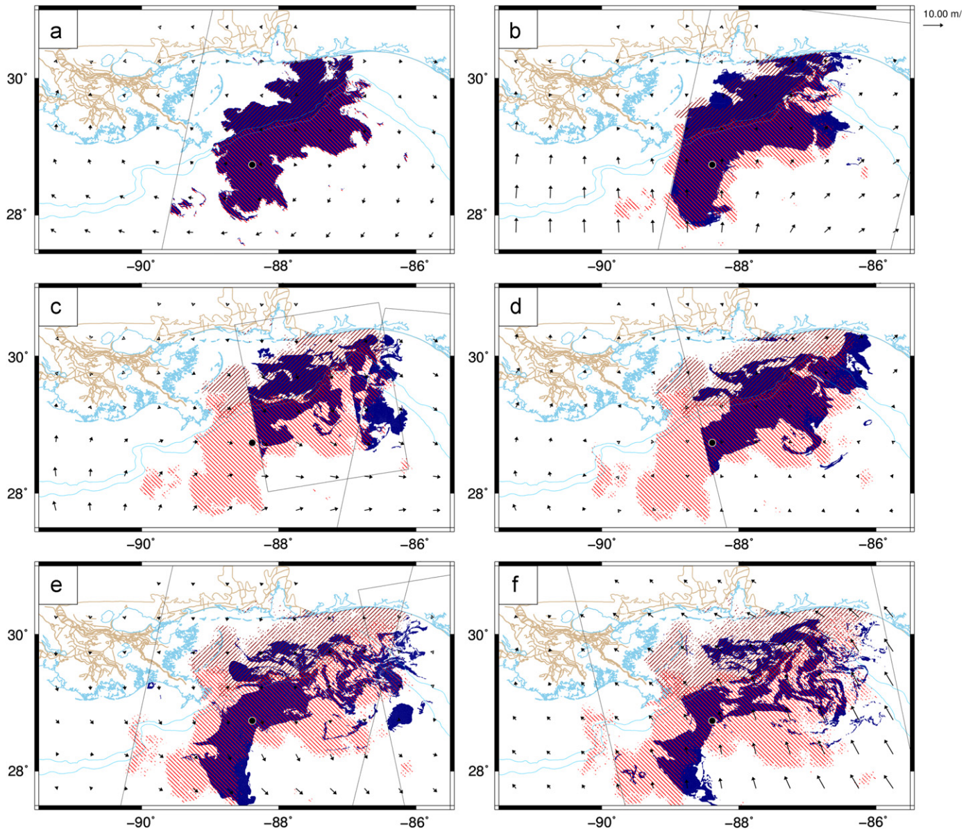
Fig. 13. Comparison of observed (solid blue) and predicted (red hatched) oil extents during the mid-June time period, with forcing with currents and winds ( F_c=1 and F_w=0.03 in Eq. (1)). A distinction is made between oil that started initially in deep water (light red hatching from northwest to southeast) and oil that started initially on the shelf (dark red hatching from northeast to southwest). The panels are (a) the initial conditions on 2010/06/13/1548UTC, (b) conditions after 44 h at 2010/06/15/1151UTC, (c) conditions after 92 h at 2010/06/17/1150UTC, (d) conditions after 132 h at 2010/06/19/0341UTC, (e) conditions after 164 h at 2010/06/20/1152UTC, and (f) conditions after 204 h at 2010/06/22/0348UTC. Vectors are wind velocities ( \text{m s}^{-1} ), and the platform location and the extents of the satellite imagery are also indicated. (For interpretation of the references to color in this figure caption, the reader is referred to the web version of this article.)
