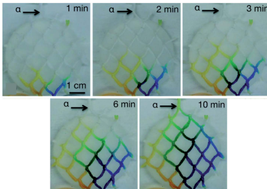
Fig. 15 Time series images showing the transport and mixing of two colored solutions, yellow and blue, through the serial dilution and combinatorial thread network, drawn from the reservoirs at the bottom of the images (one inlet thread port was immersed in each reservoir) towards the outlet at location \alpha when the SAW device placed at this location is activated. Due to the serial dilution and mixing, a stable symmetric concentration gradient across the network can be seen. Adapted from ref. 182 with permission from The Royal Society of Chemistry.
