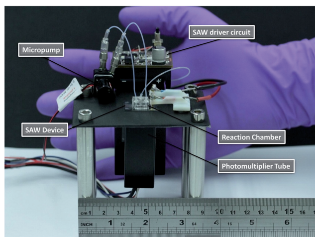
Fig. 14 Image of the proposed portable FIA system which includes a micropump, the SAW chip powered by a miniature driver circuit that includes a signal generator and amplifier, the PDMS reaction chamber bonded to the chip and a portable photodetector, showing the possibility of complete integration and portability for field use. The total weight of the entire system is approximately 130 g. Reprinted with permission from ref. 177. Copyright 2014 American Chemical Society.
