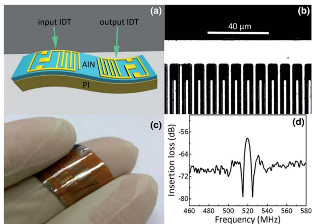
Fig. 7 (a) Schematic of the developed flexible SAW delay line device on AlN/PI composite structure, (b) microscope image of interdigital transducer fingers, (c) photographs of flexible SAW delay line devices on a PI substrate, and (d) frequency response of the flexible SAW delay line device. Used from ref. 104 with permission from Springer.
