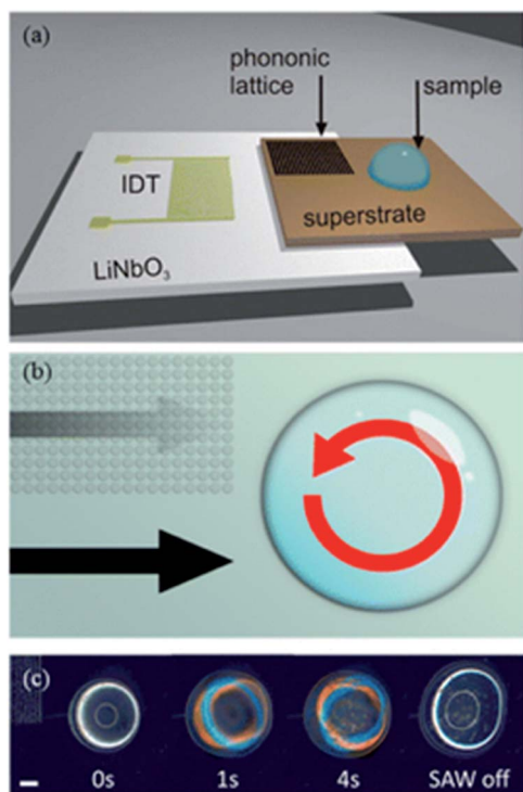
Fig. 16 Surface acoustic wave (SAW) platform used to lyse cells. (a) Device architecture showing the interdigitated transducer (IDT) used to generate the SAW on the LiNbO 3 piezoelectric wafer. The SAW is coupled into a phononic superstrate. A 20 μL droplet containing the cell suspension is deposited in the position shown. (b) The phononic lattice absorbs SAWs in a frequency-dependent manner. At ~10 MHz, propagation is hindered in regions of the lattice, whereas it is unhindered in the adjacent region. This acts to create a rotational movement within the droplet and results in shear flows that contribute to the disruption of the cell membrane. (c) The sequence of images shows a droplet of cells undergoing SAW-induced mechanical lysis. The droplet containing cells has a cloudy appearance, which is observed to become largely clear upon successful lysis of cells. Note that the colored rings observed in part of the image sequence are an optical effect of the stereomicroscope used to observe lysis. Scale bar 1 mm. Reprinted with permission from ref. 188. Copyright 2015 American Chemical Society.
