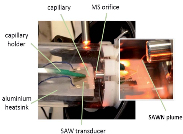
Fig. 10 Photograph showing coupling of the SAWN ionization device to an LC capillary at the inlet of a mass spectrometer. Reproduced from ref. 149 with permission from Wiley.
