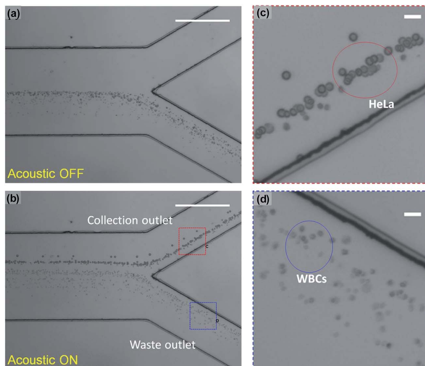
Fig. 12 Micrographs of the separation process with acoustic field ON and OFF. (a) The mixture of HeLa cells and WBCs through a microfluidic channel with the acoustic field OFF. All of the cells were directed to the lower waste outlet by the hydrodynamic flow. No separation is observed. (b) When the acoustic field is ON, larger HeLa cells were pushed to the collection outlet, whereas the smaller WBCs still remained in the waste outlet. The separation between HeLa cells and WBCs can be observed. The stacked images are from 50 consecutive frames (scale bars, 515 \mu\text{m} ). (c and d) Zoomed-in images of the collection outlet and the waste outlet, respectively (scale bars, 30 \mu\text{m} ). Adapted from ref. 158, courtesy National Academy of Sciences.
