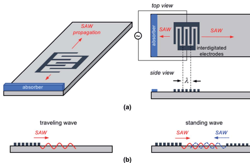
Fig. 1 (a) Schematic of a single, planar IDT configuration, where the SAW propagates away from the IDT in both directions. Typically, an absorbent material such as a gel is used to inhibit reflection of the backward traveling SAW. The top and side views show a typical IDT structure with the interdigitated electrode fingers spaced \lambda/2 . (b) Side views to two common actuation strategies. On the left is a traveling wave configuration, where a single IDT induces a SAW propagating away from the electrodes. Generally, the SAW propagates at the speed of sound of the crystal, which is typically \sim 10^3 \text{ m s}^{-1} , but has an out-of-plane displacement amplitude of only \sim 10 \text{ nm} . However, the displacement speed and acceleration can be very high, \sim 1 \text{ m s}^{-1} and 10^5 \text{ m s}^{-2} . On the right are two sets of IDTs that generate counter-propagating SAWs. The SAWs interfere to form a standing wave.
