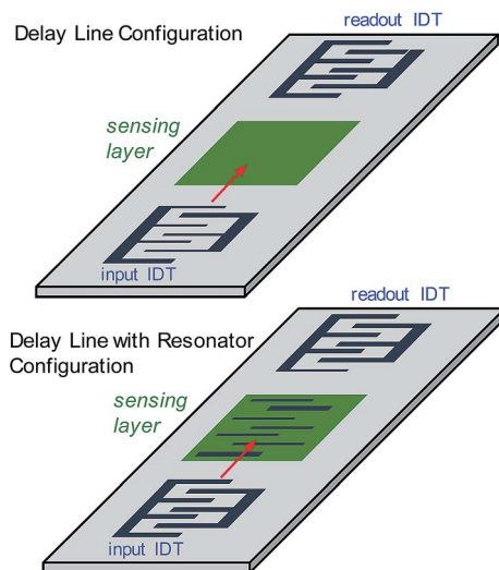
Fig. 2 Two common configurations using a pair of IDTs for sensing applications. On the top is the delay line configuration, where a SAW is produced at the input IDT and as it travels through the sensing layer, interactions with adsorbed targets induce a frequency shift that can be detected at the readout IDT. On the bottom is a similar configuration but with additional IDT electrodes beneath the sensing layer. This resonator IDT acts as a reflector to set up a resonant cavity and increase sensitivity.
