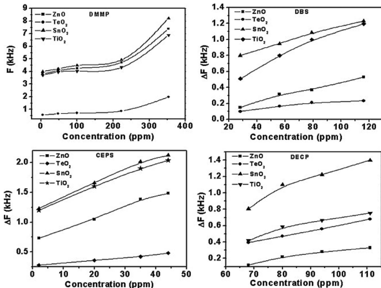
Fig. 4 Variation in differential frequency shifts ( \Delta F ) of SAW E-nose as a function of the concentration of different simulants of CWA on four different oxide sensing layers – ZnO, tellurium dioxide (TeO 2 ), tin dioxide (SnO 2 ), and titanium dioxide (TiO 2 ). Upper left – dimethyl methyl phosphonate (DMMP), upper right – dibutyl sulfide (DBS), lower right – diethyl chlorophosphate (DECP), lower left – chloroethyl phenyl sulfide (CEPS). Adapted from ref. 72 with permission from Elsevier.
