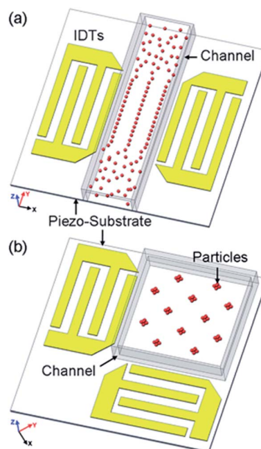
Fig. 11 Schematic of the SAW-based patterning devices. (a) 1D patterning using two parallel IDTs. (b) 2D patterning using two orthogonal IDTs (the angle between the IDTs can be changed to achieve different patterns). Reproduced from ref. 151 with permission from The Royal Society of Chemistry.
