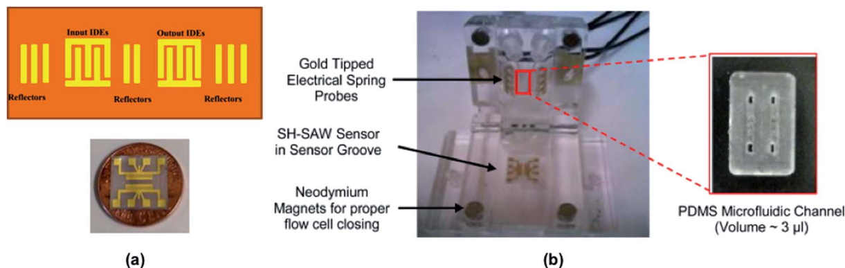
Fig. 5 (a) Schematic of the SH-SAW device (top) and the as-fabricated SH-SAW sensor on a U.S. penny for reference (bottom). (b) Flow cell with the SH-SAW sensor in the sensor groove (inset: PDMS microfluidic flow channel). A chemical sensing layer, naphtho[2,3- a ]dipyrido[3,2- h :2',3'- f ]phenazine-5,18-dione (QDPPZ), was synthesized and employed for the selective detection of lead nitrate ( \text{PbNO}_3 ) and cadmium nitrate ( \text{CdNO}_3 ) down to pM-level concentrations. Adapted from ref. 84 with permission from Elsevier.
