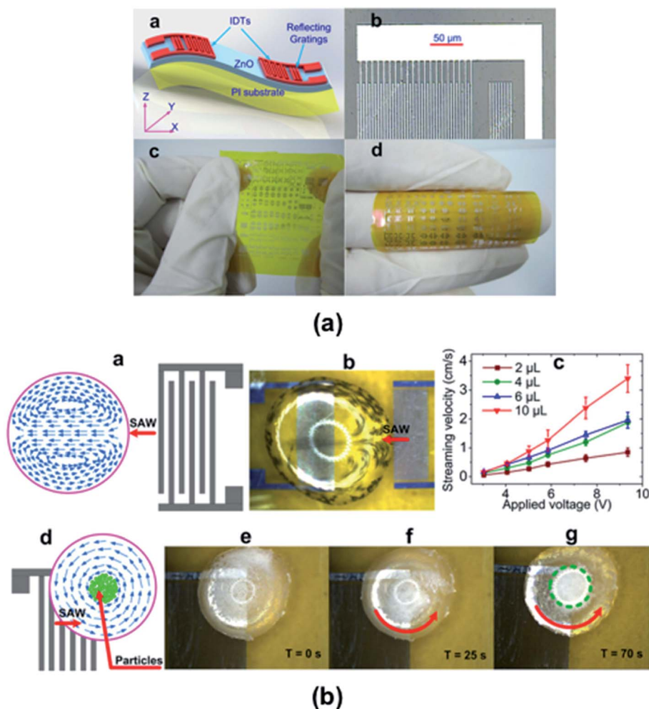
Fig. 6 (a) Schematic of the flexible thin film ZnO/polyimide SAW devices and photographs of the IDT design and fabricated devices. (b) Schematics and photographs of induced acoustic streaming in a surface droplet along with measurements of the streamlining velocity as a function of the applied voltage and images showing the concentration of particles in the droplet. Adapted with permission from Macmillan Publishers Ltd: ref. 103, 2013.
