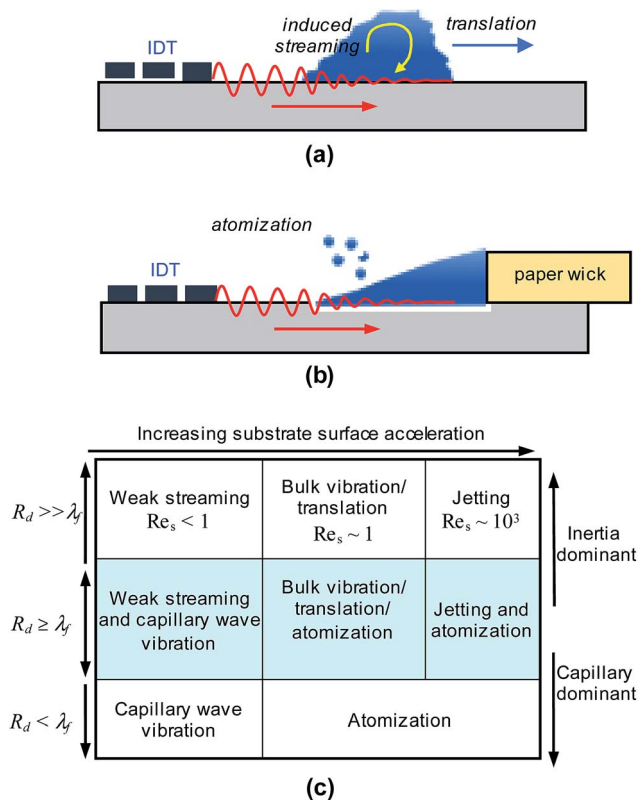
Fig. 8 (a) Induced streaming due to the acoustic pressure of the refracted SAW wave into a surface droplet. In this traveling wave configuration, the droplet can translate or, at sufficient SAW amplitude, break-up and be ejected from the surface. (b) A 'pinned' droplet configuration, where solution is fed from a paper wick connected to an external solution reservoir. A thin film of fluid is extracted from the wick onto the surface of the SAW device. Similar to the surface droplet configuration, at sufficient SAW amplitude the extracted film is atomized. (c) The modes of liquid break-up depending on the relative size of the droplet on the surface of the substrate ( R_d ) and the acoustic wavelength in the fluid ( \lambda_f ). The streaming Reynolds number ( Re_s ) is a non-dimensional number characterizing the inertia of the streaming fluid to viscous effects. Table adapted with permission from ref. 109. Copyrighted by the American Physical Society.
