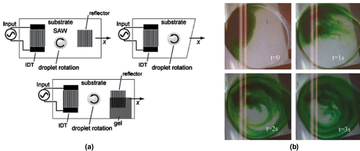
Fig. 13 (a) Schemes for symmetry breaking of SAW propagation in order to generate azimuthal liquid recirculation. The left picture shows one of the IDTs partly covered with \alpha -gel damping material and the right picture shows the use of only one IDT with the wafer cut in a diagonal fashion. (b) Images at 60 frames per s showing the visualization of azimuthal bulk recirculation generated by asymmetric SAW propagation through dye streamlines induced by the flow. Adapted from ref. 167 with permission from Springer.
