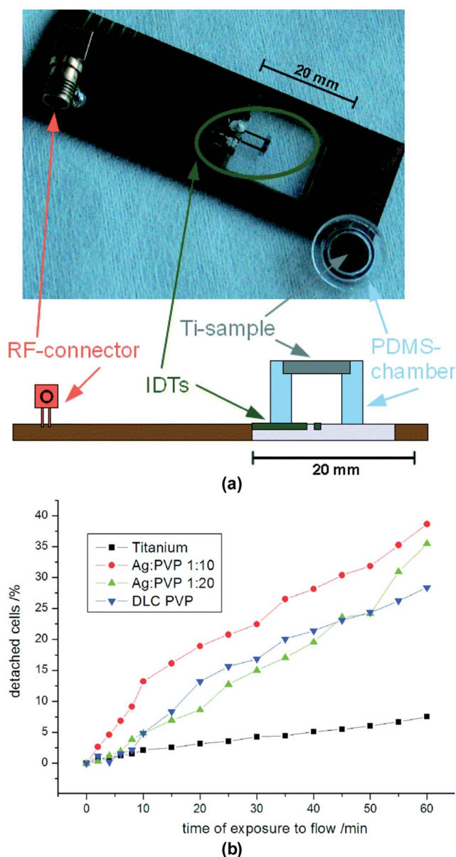
Fig. 17 (a) Photograph (top) and schematic cross-section (bottom) of the setup for cell adhesion measurements. The system consists of a transparent piezoelectric LiNbO 3 substrate with interdigital transducers (IDTs, green-brown color in the figure). On top of the substrate and the IDTs, a polydimethylsiloxane (PDMS)-chamber (blue) is placed which is covered by the implant specimen, in this case a titanium sample (grey). In the top photograph, the PDMS-chamber (upside-down) is removed from the LiNbO 3 substrate, whereas the cross-section in the bottom part of the figure shows the system in its closed and assembled configuration. The electrical radio-frequency (rf) connector is labeled in orange. It is connected to the IDTs via silver conductive paste and two separated Cu-parts on the chip-carrier. (b) Percentage of detached SAOS-2 cells on different samples as marked by different symbols after 60 minutes of initial adhesion time versus time of flow exposure. Titanium exhibits the smallest de-adhesion rate as compared to the different DLC surfaces. Within this set of substrates, the de-adhesion tendency increases with higher silver-doping. Reproduced from ref. 191 with permission from The Royal Society of Chemistry.
