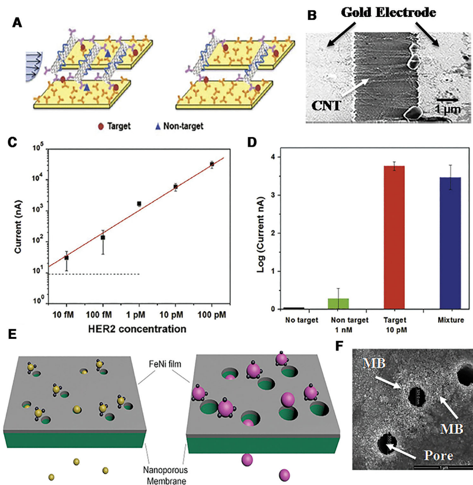
Figure 7. (A) Schematic of irreversible hydrodynamic shearing of non-specifically bounded CNTs. (B) Trapping of CNTs across a 3-micron gap by a DC and AC protocol. (C) Using an optimized shear protocol, we can detect HER2 marker at concentrations (10 fM) orders of magnitude lower than its dissociation constant at nM and (D) selective detection of HER2 in the presence of a 100 times more abundant isoform in serum. (Reproduced from [57] with permission. (E) Schematic of nanomagnetic bead trapping. (F) The high magnetic field gradient at the pore tip of a track-etched membrane coated with a Fe/Ni film can also trap magnetic bead (MB) particles.
