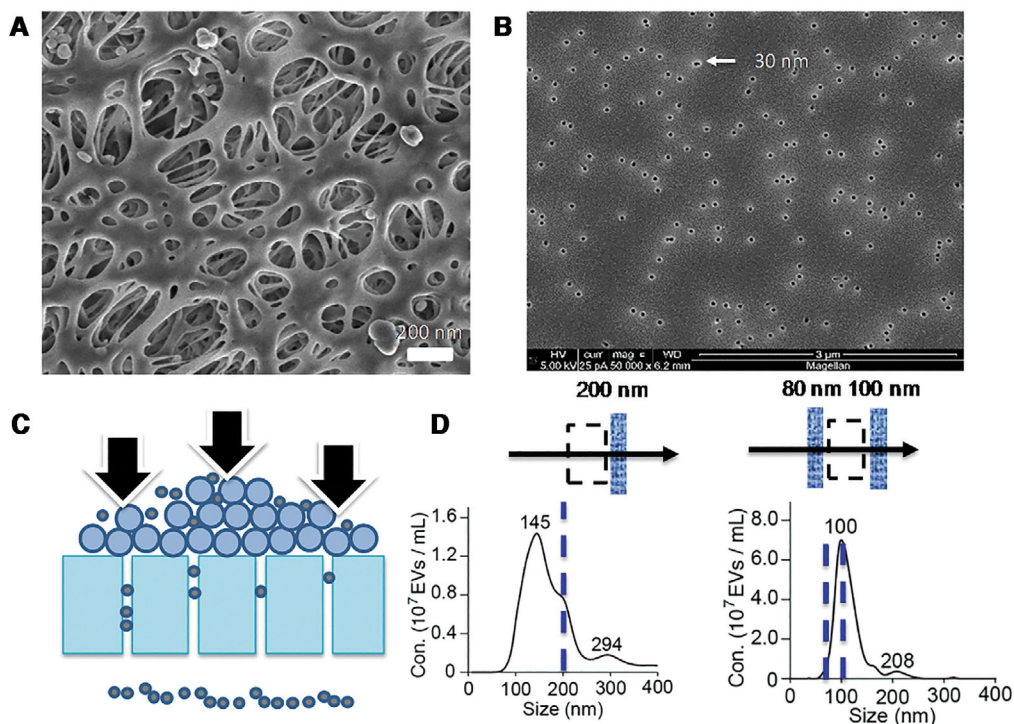
Figure 5. Representative EM images of (A) an ultrafiltration polyethersulfone (PES) membrane showing irregular pores with different radii and (B) our track-etched membranes with uniform pore radius. Fractionation of cell culture media using track-etched membranes show significant filter cake formation and EV coalescence as schematically shown in (C) that results in a poor size fractionation and leads to particles about twice the average EV size in the flow through (D) (Reproduced from Supplementary Materials of [42] with permission). These large particles are larger than the pore size by 100 nm and hence are believed to be created by coalescence events in the pore.
