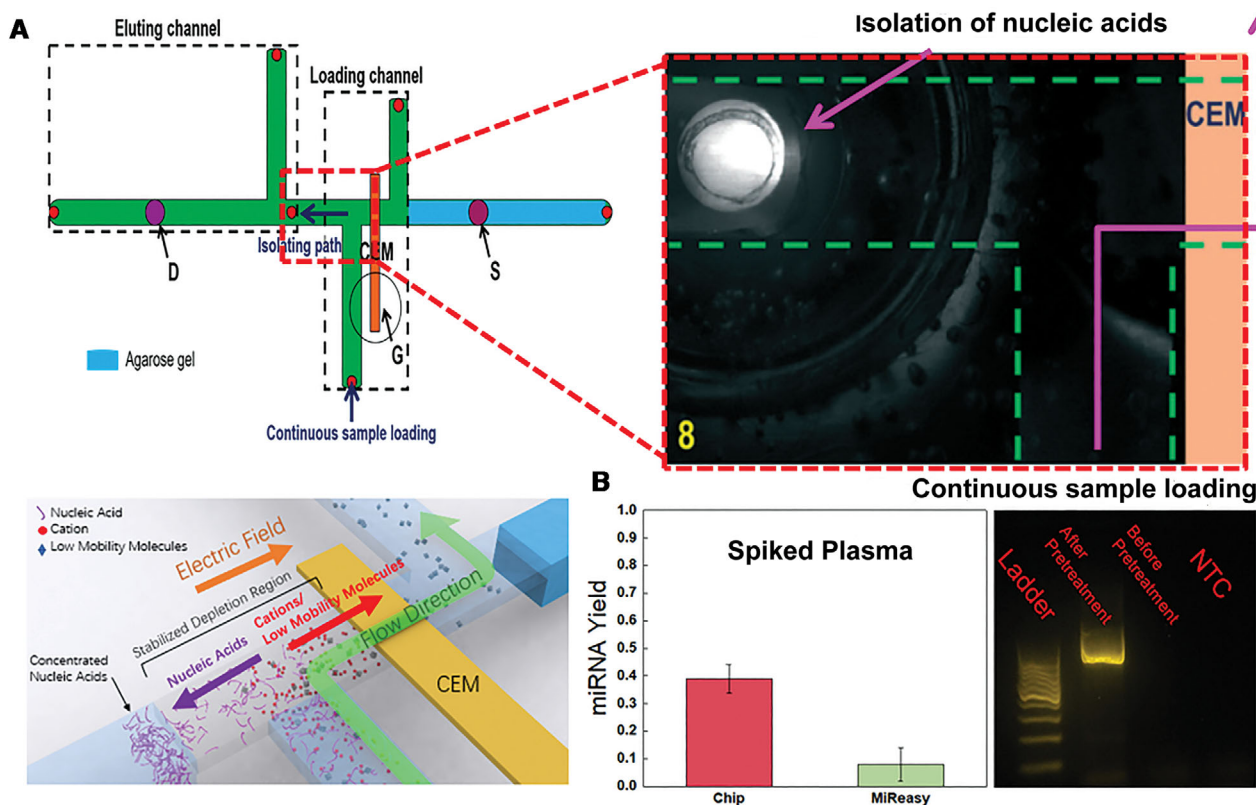
Figure 3. (A) A depletion front generated by the ion-exchange membrane G extends to the junction between the two cross-channels, the bottom vertical channel and the horizontal channel. Spiked DNA serum flows from the bottom vertical channel to the right of the horizontal channel before exiting by another vertical channel, as shown by the blue line. The high field in the junction extracts the DNA and places it in a buffer to the left of the horizontal channel. (B) Spiked microRNA and DNA into serum is tested with the pretreatment chip. The reverse-transcription PCR yield of microRNA is shown to be more than 4 times higher than the best commercial pretreatment unit. There is no PCR amplification of the DNA without pretreatment (Reproduced from [10] with permission from the Royal Society of Chemistry).
