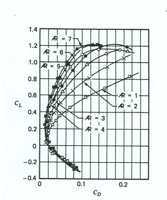
Figure 2: Experimental test for calculated C_{D_i} for rectangular wings of 1 \leq AR \leq 7 (Prandtl, 1921).
