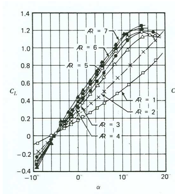
Figure 1: Experimental test for calculated C_L for rectangular wings of 1 \leq AR \leq 7 (Prandtl, 1921).
