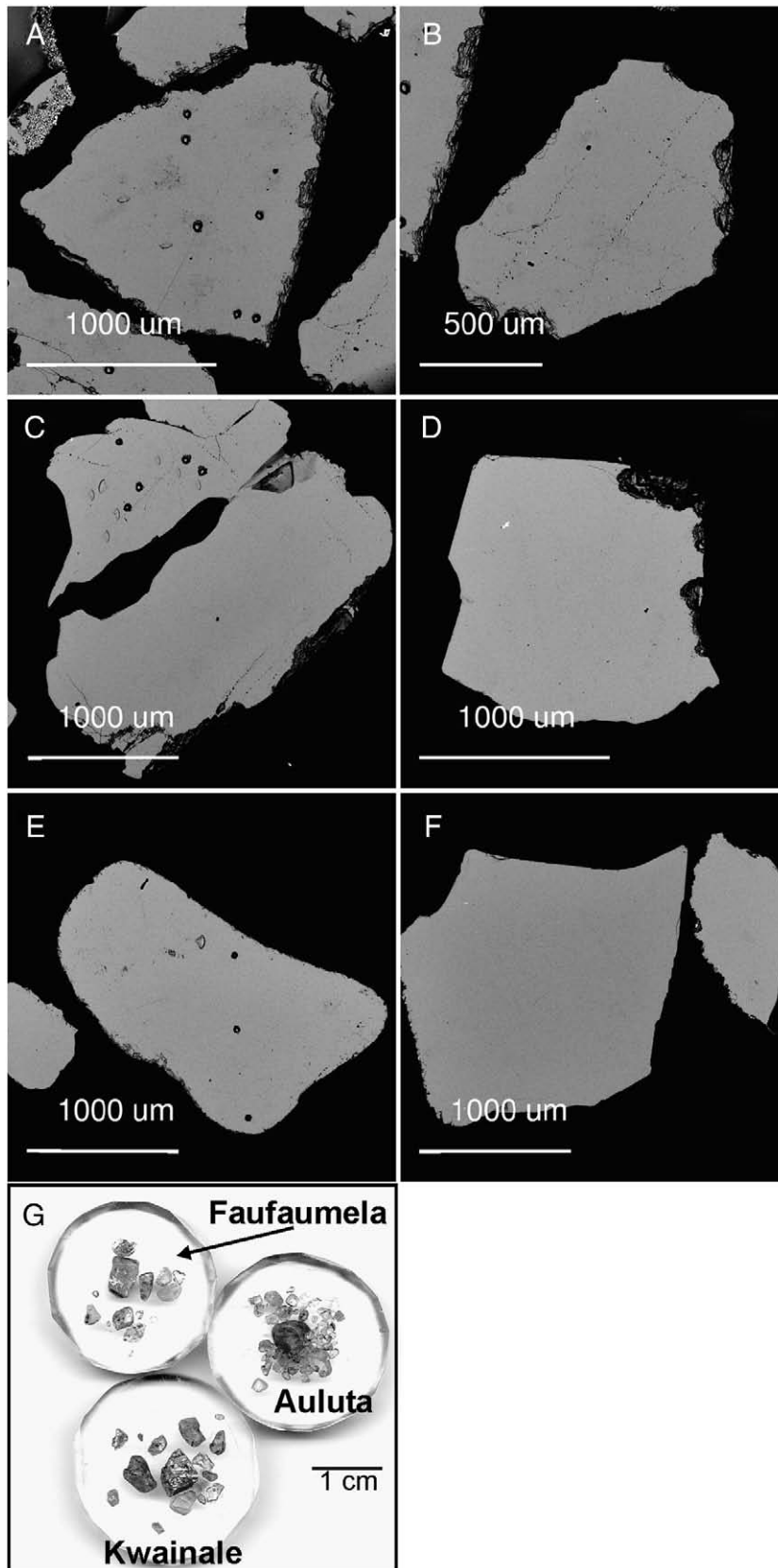
Fig. 2. Back scattered electron images of Malaitan zircon megacrysts: A- A1-Z3, B- A1-Z6, C- F1-Z1, D- F1-Z5, E- K1-Z1, F- K1-Z5. The small pits in several of the grains indicate locations of laser ablation spots (40 μm) for trace element analysis. G- Photo exhibiting the three epoxy mounts containing the megacryst zircon grains from Auluta, Faufaumela, and Kwainale.
