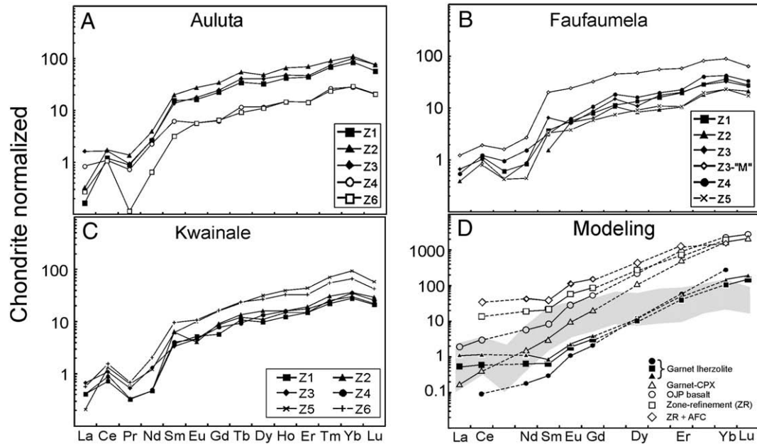
Fig. 4. Chondrite-normalized REE plots for zircons from (A) Auluta, (B) Faufaumela, and (C) Kwainale exhibiting the average compositions for all of the grains analyzed in this study (Table S1). Chondrite values are from Palme and Jones (2005) . D) Plot illustrating the chondrite-normalized REE patterns for calculated zircon compositions in equilibrium with various melts/mantle source using the partition coefficients of Irving and Frey (1984) . Solid circle = depleted asthenospheric mantle, open square = zone-refined melt, and open diamond = final anorthite melt subsequent zone refinement and fractional crystallization (all from Neal and Davidson, 1989 ); open triangle = clinopyroxene-garnet mantle xenolith from Ishikawa et al. (2007) ; open circle = OJP basalt from Mahoney et al. (1993) ; solid square = high-temperature garnet lherzolite and solid triangle = low-temperature garnet lherzolite from Schmidberger and Francis (1999) and Schmidberger et al. (2001) . See text for detailed discussion.
