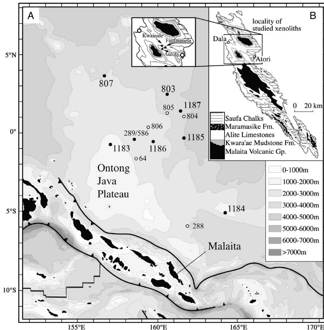
Fig. 1. A) Bathymetric regional map of the main part of the Ontong Java Plateau and location of Solomon Islands volcanic arc chain (modified after Ishikawa et al., 2004). Numbered sample locations within OJP indicate ocean drilling program (ODP), with solid circles representing sites that have intersected basement. B) Inset illustrates simplified geological map of Malaita (after Petterson, 1995) indicating sample locations.
