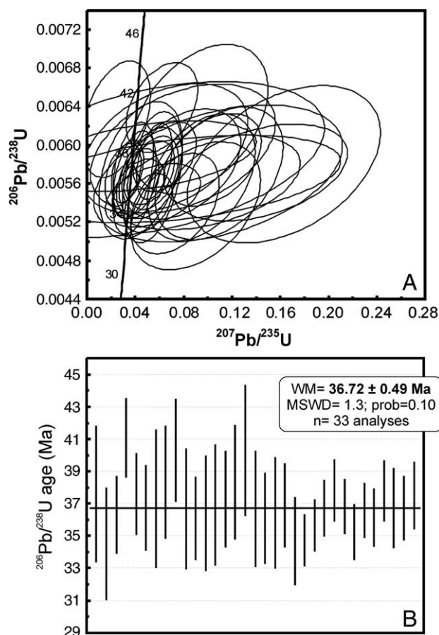
Fig. 7. A- Concordia plot showing the individual U–Pb laser ablation analyses for Kwainale megacryst zircons analyzed (Table S3c); B- Diagram illustrating the distribution of WM ^{206}\text{Pb}/^{238}\text{U} ages determined for individual Kwainale zircon megacrysts. WM ages were calculated using IsoPlot/Ex3.00 (Ludwig, 2003).
