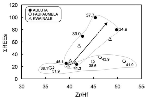
Fig. 3. Plot showing variation of REEs vs. average Zr/Hf ratios for Malaitan zircon megacrysts. The zircon megacrysts from Auluta (solid circles) indicate a positive correlation between REEs and increasing Zr/Hf ratios and decreasing WM ^{206}\text{Pb}/^{238}\text{U} ages (data point labels), whereas the same parameters do not correlate with age determinations for the Faufaumela zircons (open circles).
