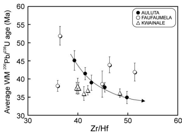
Fig. 9. Diagram illustrates the variation between average Zr/Hf values and calculated WM ^{206}\text{Pb}/^{238}\text{U} ages for Malaitan zircons. The negative correlation may reflect zircon formation from a mantle source undergoing progressive carbonate/ \text{CO}_2 -dominated metasomatism (see text for details).
