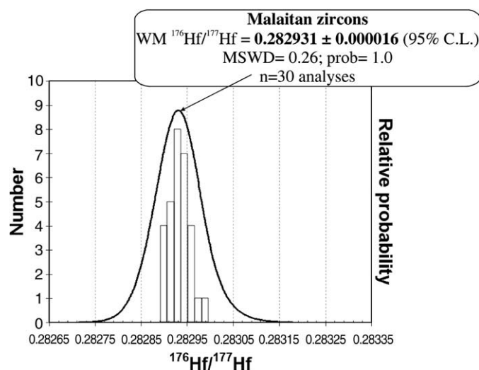
Fig. 8. Probability density plot illustrating the distribution of in-situ ^{176}\text{Hf}/^{177}\text{Hf} values obtained for Malaitan zircon megacrysts analyzed (Table S4). Plot and weighted mean calculations conducted using IsoPlot/Ex3.00 (Ludwig, 2003).
