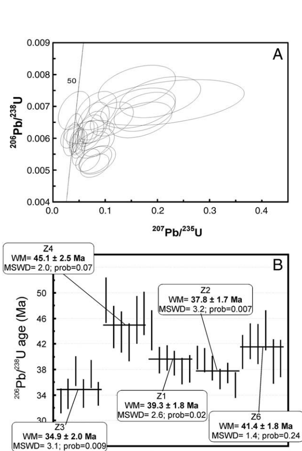
Fig. 5. A- Concordia plot showing the individual U-Pb laser ablation analyses for Auluta megacryst zircons analyzed (Table S3a); B- Diagram illustrating the distribution of the WM ^{206}\text{Pb}/^{238}\text{U} ages determined for individual Auluta zircon megacrysts. WM ages were calculated using IsoPlot/Ex3.00 ( Ludwig, 2003 ).
