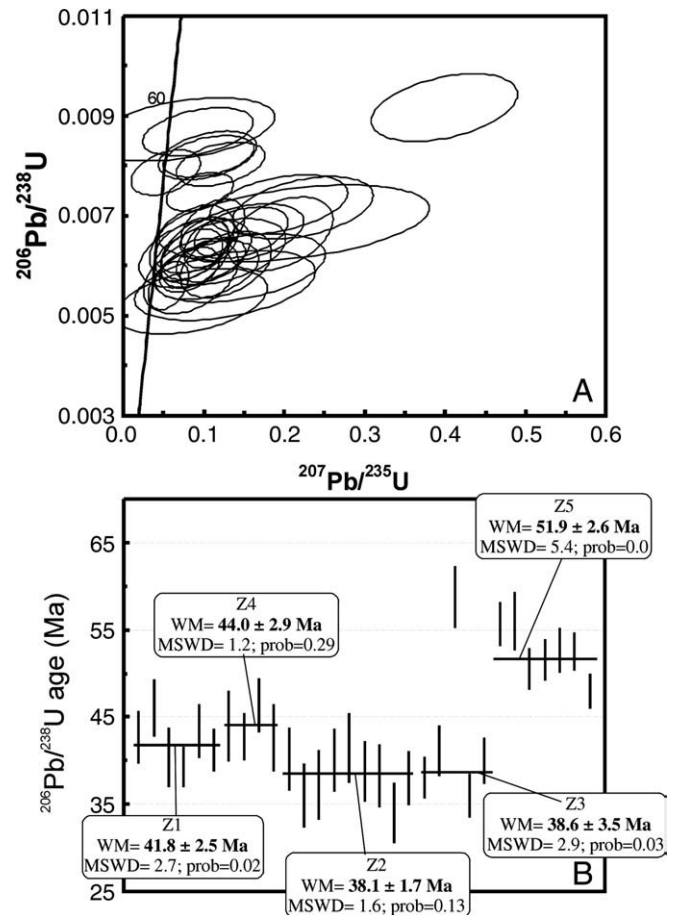
Fig. 6. A- Concordia plot showing the individual U-Pb laser ablation analyses for Faufaumela megacryst zircons analyzed (Table S3b); B- Plot illustrating the distribution of the WM ^{206}\text{Pb}/^{238}\text{U} ages determined for individual Faufaumela zircon megacrysts. WM ages were calculated using IsoPlot/Ex3.00 ( Ludwig, 2003 ).
