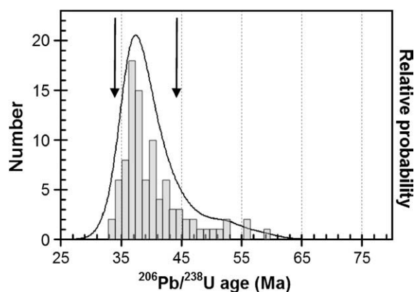
Fig. 10. Probability density plot exhibiting the distribution of calculated WM ^{206}\text{Pb}/^{238}\text{U} ages for Malaitan zircon megacrysts analyzed in this study (Table S3). The arrows indicate previous age determinations for a phlogopite grain from a mantle xenolith at 34 Ma (Ar–Ar; Kelley and Wartho, 2000), 33.9 Ma WM ^{206}\text{Pb}/^{238}\text{U} age for a single zircon megacryst from Malaita (Davis, 1978), and the 44.2 \pm 0.2 Ma Ar–Ar age for basalts belonging to the younger series and Northern Malaita Alkaline Suite (NMAS; Tejada et al., 1996).
