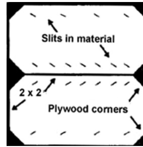
Fig. 6–5. Homemade 12x12 inch square benthic barrier constructed of 2x2 inch, non-pressure-treated wood. (ADAPTED
